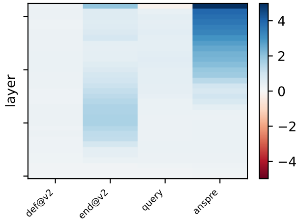
llama31-8b direct: \log p(\text{true}) - \log p(\text{lure})
