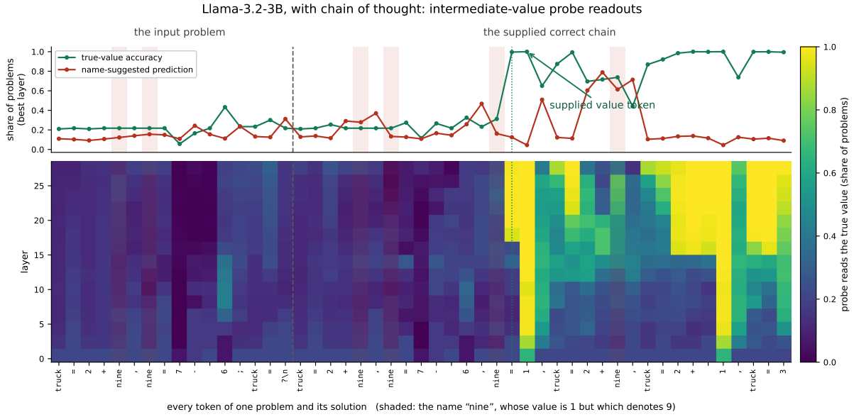
Figure 6: Llama-3.2-3B intermediate-value readouts under supplied correct calculations. Rates pool problems; tokens illustrate one example.
