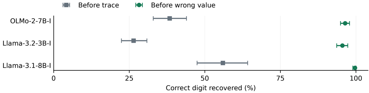
Figure 3: Correct digits are recoverable immediately before actual wrong writes (95% intervals).
