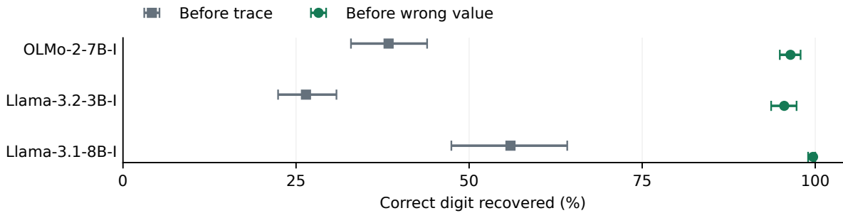
Figure 3: Correct digits are recoverable immediately before actual wrong writes (95% intervals).
