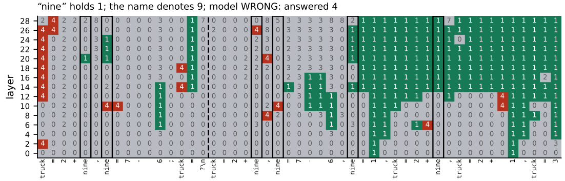
Figure 18: As above, for the intermediate variable. Red is the model’s final answer, which is the queried variable’s value, so a cell that matches it is not a readout of this variable.
