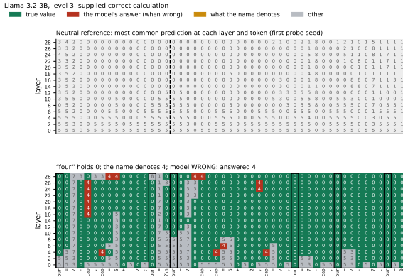
Figure 4: Adapted from Kudo et al.’s Figure 3. Probes read a supplied correct calculation for a problem the model answers with the name-suggested digit. Bottom: majority prediction over three probe seeds at each layer and token; green the variable’s true value, red the value the model answered, amber the value its name denotes, grey anything else. Top: the most common prediction on neutral problems from the first probe seed, for reference. Boxes mark name tokens; the dashed line marks the calculation’s start. Matching the neutral reference alone does not establish a cell’s information content.
