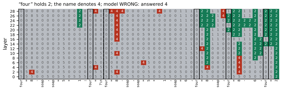
Figure 15: A third problem answered with the name-suggested value.
