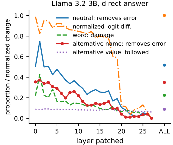
Figure 2: Llama-3.2-3B, answer-only: queried-variable name errors removed by layer, with neutral-word damage and alternative-name controls. Removal counts changes away from the name-suggested digit.
