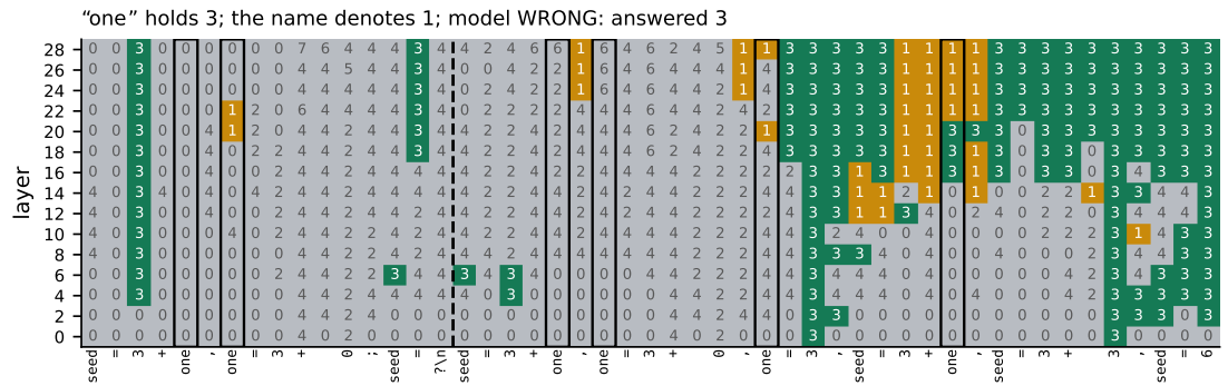
Figure 19: A second problem, intermediate variable.
