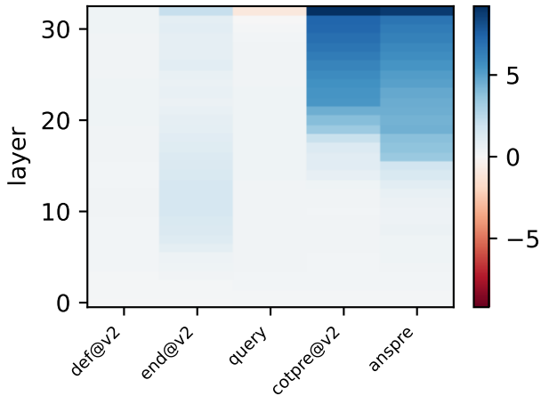
llama31-8b cot: \log p(\text{true}) - \log p(\text{lure})
