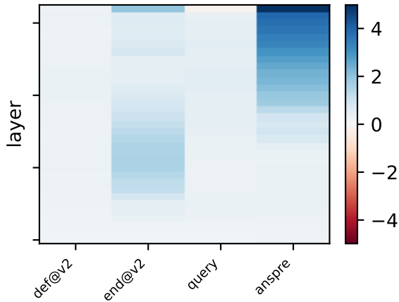
llama31-8b direct: \log p(\text{true}) - \log p(\text{lure})
