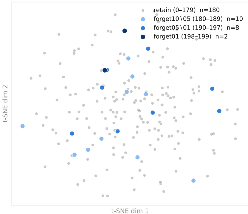
TOFU per-author LoRA deltas (n=200, perplexity 30)
