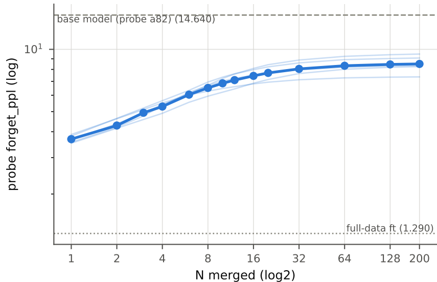
own-author perplexity
