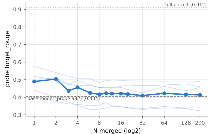
own-author ROUGE-L recall
