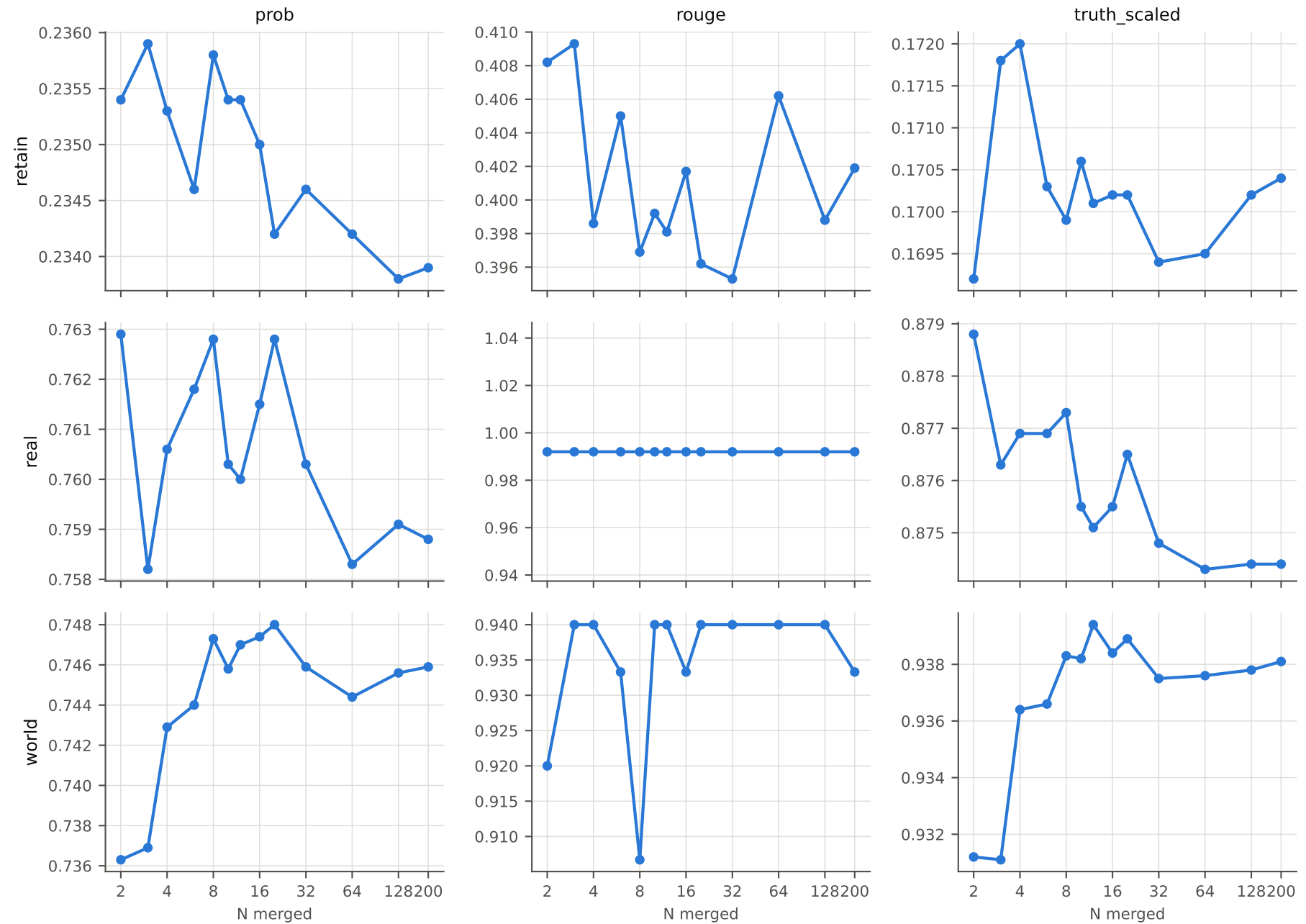
model_utility components vs N — retain coverage rises, does real/world pay?
