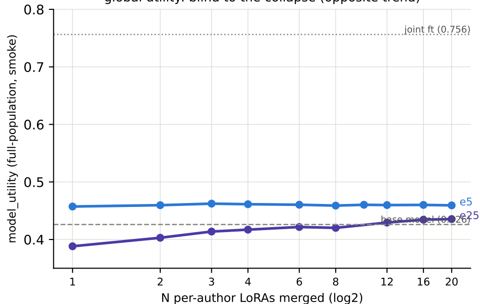
global utility: blind to the collapse (opposite trend)
