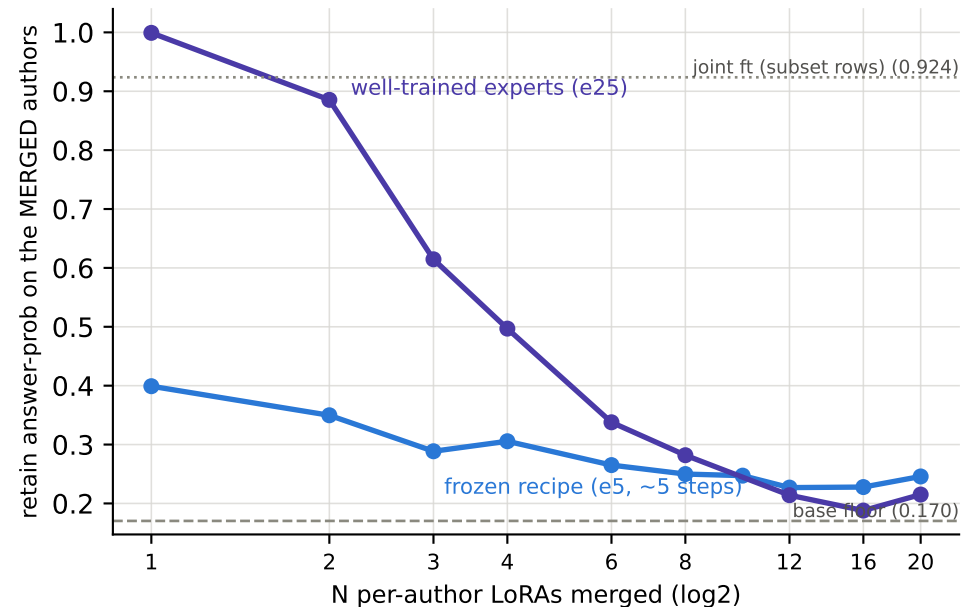
what it was trained on: collapse, same knee N \approx 3
