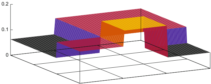
Fig. 7.2 Stationary distribution on the maze (5.3.7)
