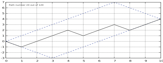
Fig. 3.1 Graph of 120 = \binom{10}{7} = \binom{10}{2} paths with n = 5 and k = 2
