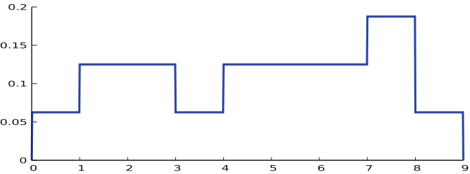
Fig. 7.3 Stationary distribution by state numbering
