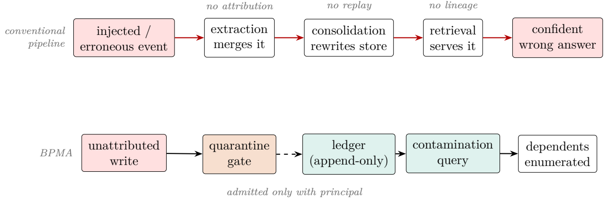
Figure 3: Failure cascade. Top: in a mutable pipeline one bad write propagates through extraction, consolidation, and retrieval, and the trail is destroyed behind it. Bottom: BPMA quarantines unattributed writes at entry, and when a source is later found bad, a contamination query enumerates every Claim derived from it.
