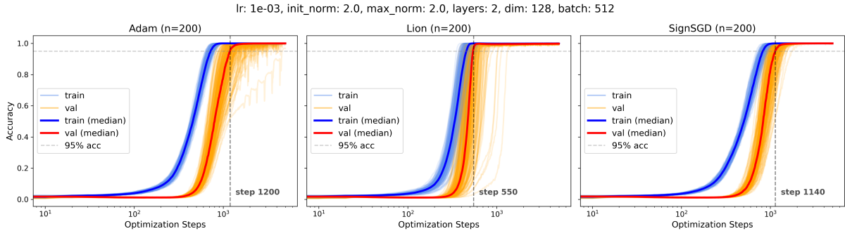
Figure 3: Multi-seed accuracy on the 2-layer architecture ( init_norm=2.0 , max_norm=2.0 , n=200 ). Dashed lines mark median steps to 95% val accuracy: Adam 1,200 ( \text{lr}=10^{-3} ), Lion 550 ( \text{lr}=10^{-3} ), SignSGD 1,140 ( \text{lr}=10^{-3} ). All seeds converge within 5,000 steps with zero failures.
