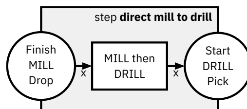
Figure 3.29: Direct Module Interaction Modelling Approach
