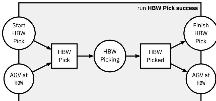
Figure 3.5: HBW Pick run (Store into HBW)
