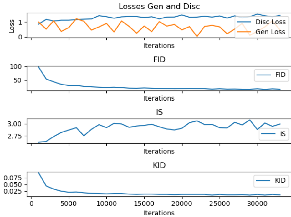
Figure 1: Training of first configuration not further specialized
