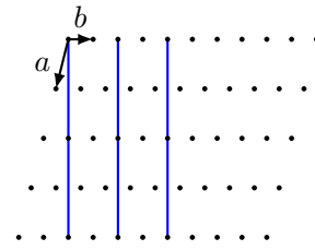
(c) 1\bar{2}0
