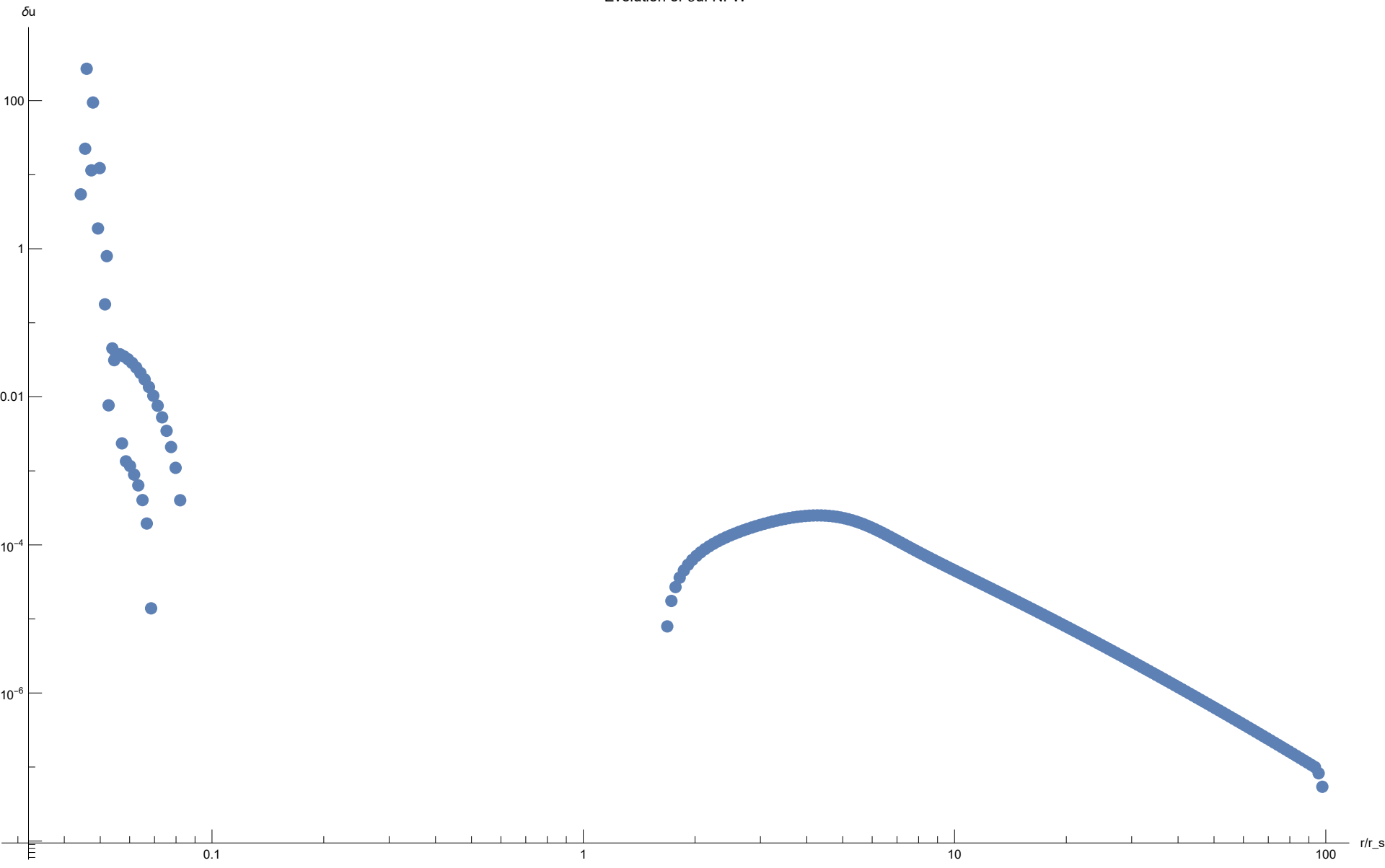
Evolution of \delta u : NFW
