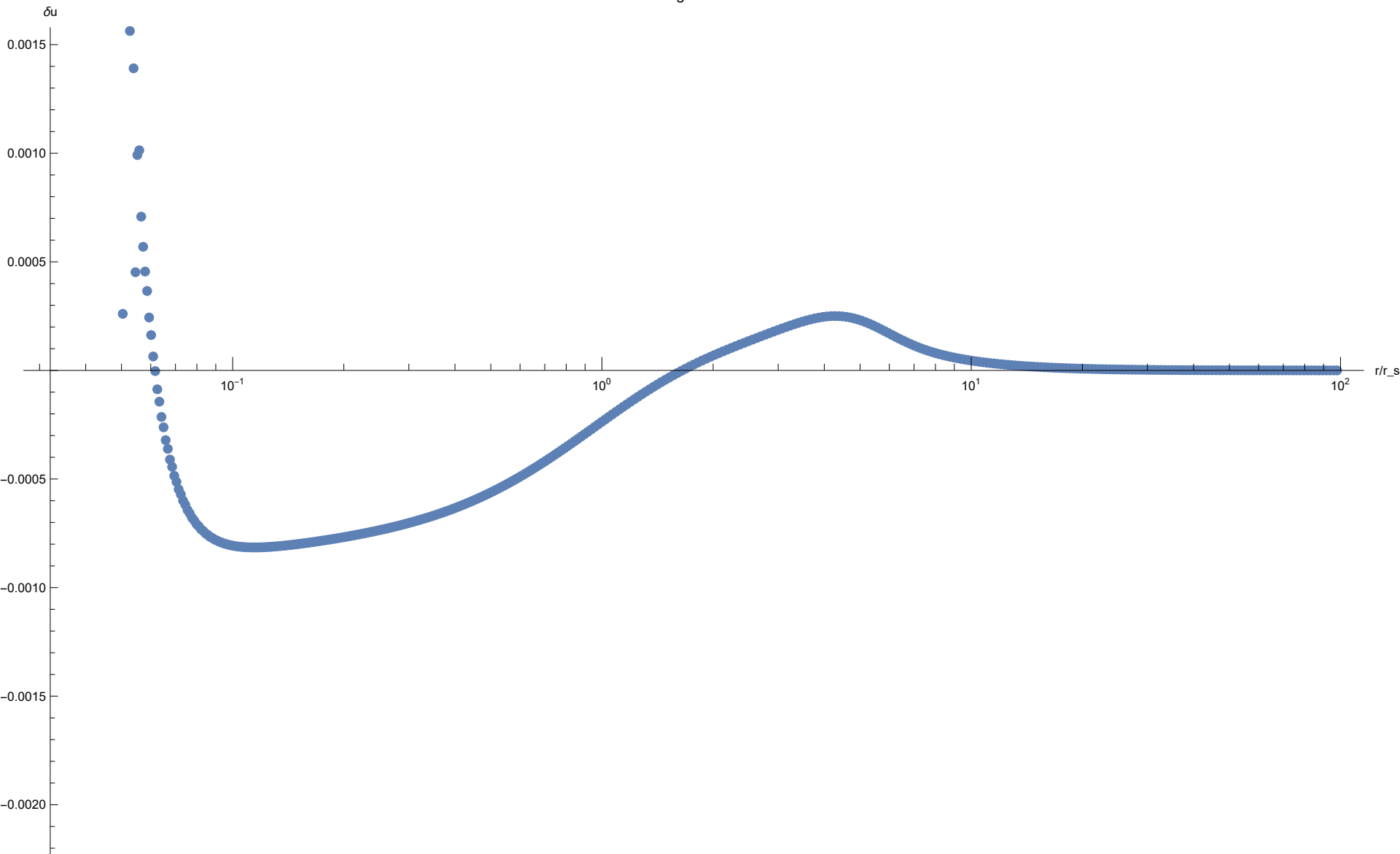
Plot with Logarithmic X-Axis
