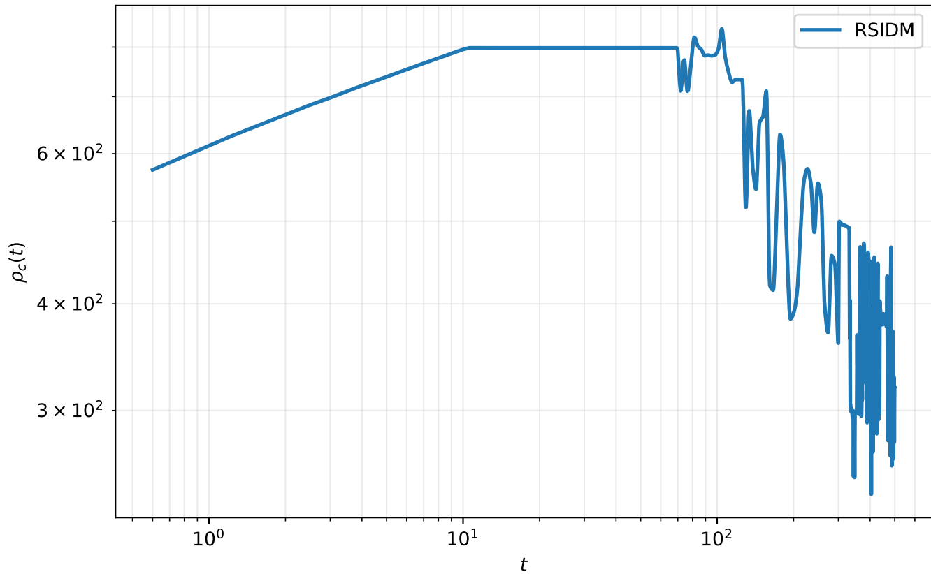
Central density evolution
