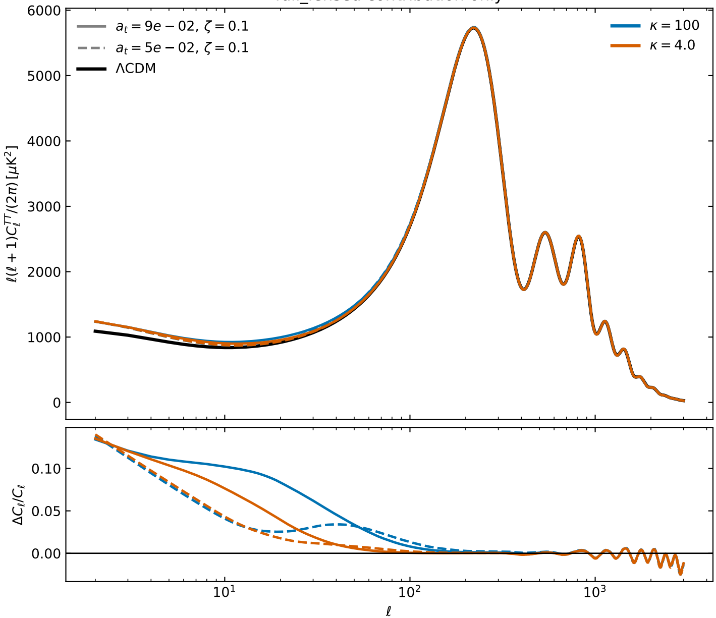
full_lensed contribution only
