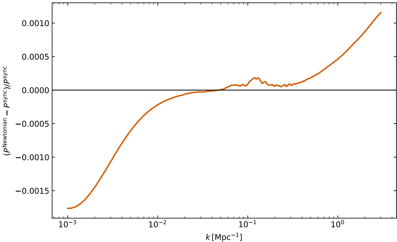
Gauge test: matter power spectrum
