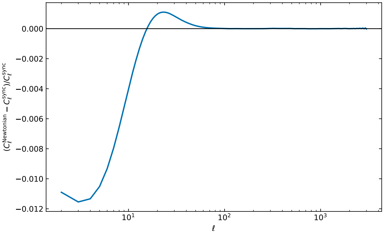
Gauge test: TT spectrum
