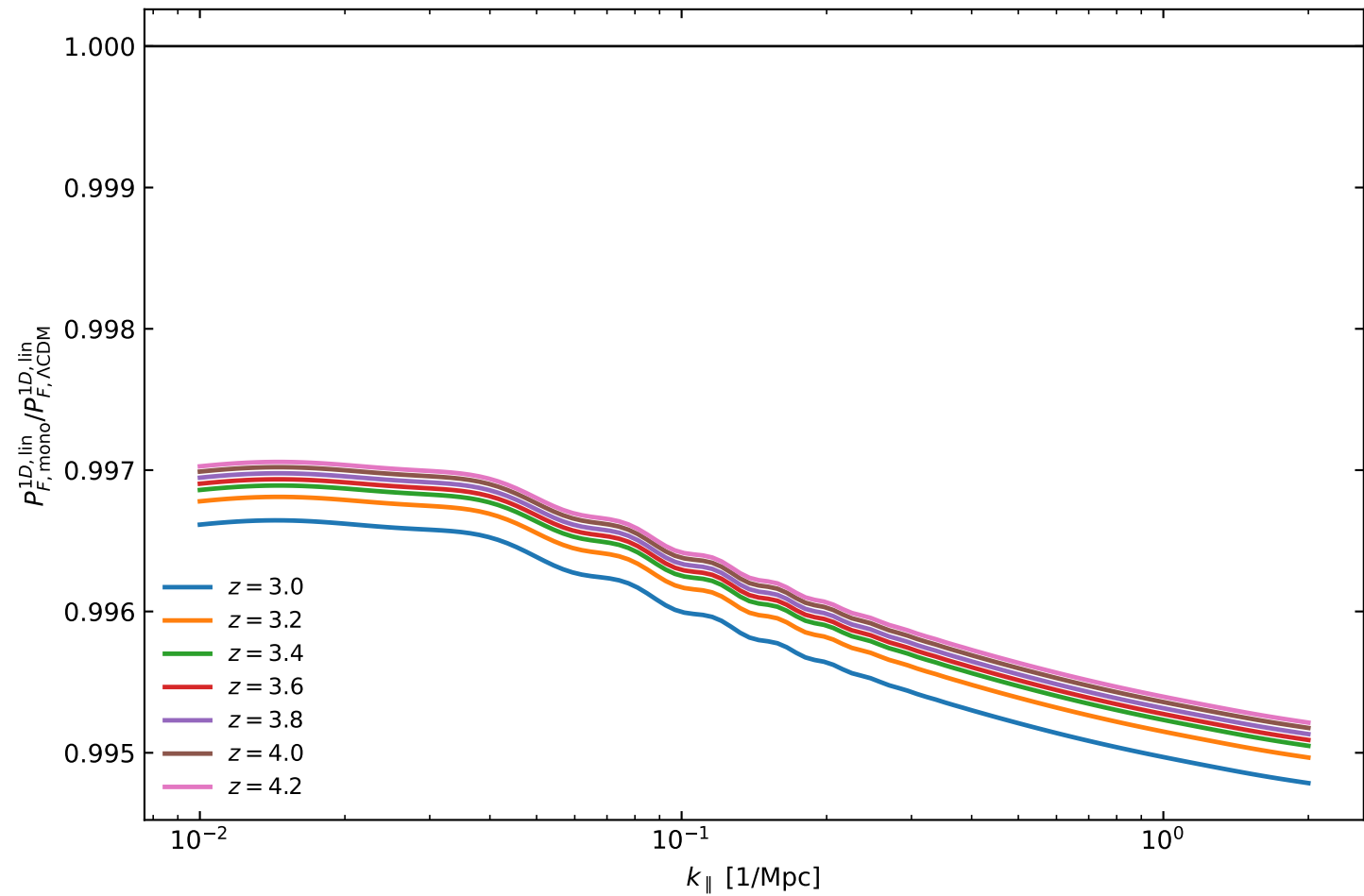
Linear Ly \alpha proxy: Instantaneous, a_t = 0.25 , f_{\text{mon}} = 0.05
