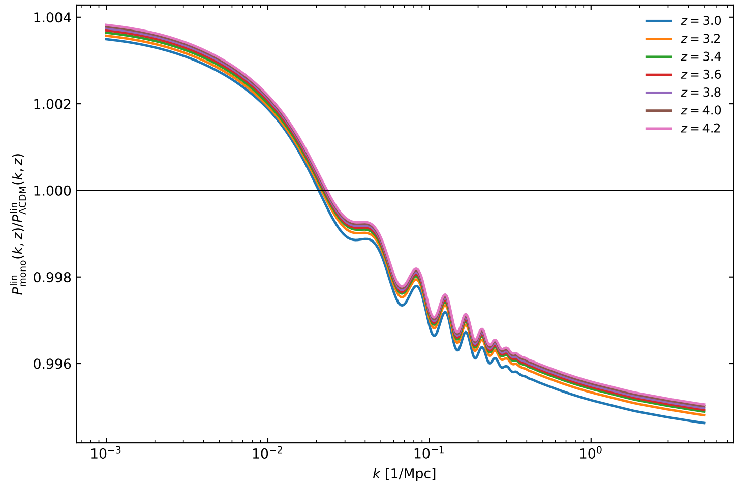
Linear matter ratio: Intantenous, a_t = 0.25 , f_{\text{mon}} = 0.05
