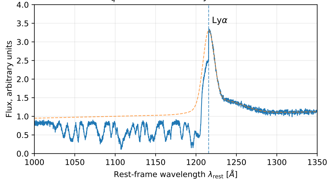
z_q < 6 : transmitted Ly \alpha forest
