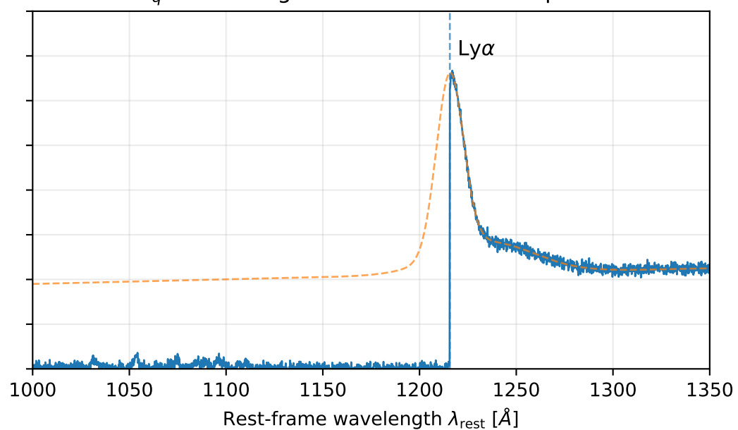
z_q > 6 : strong Gunn--Peterson absorption
