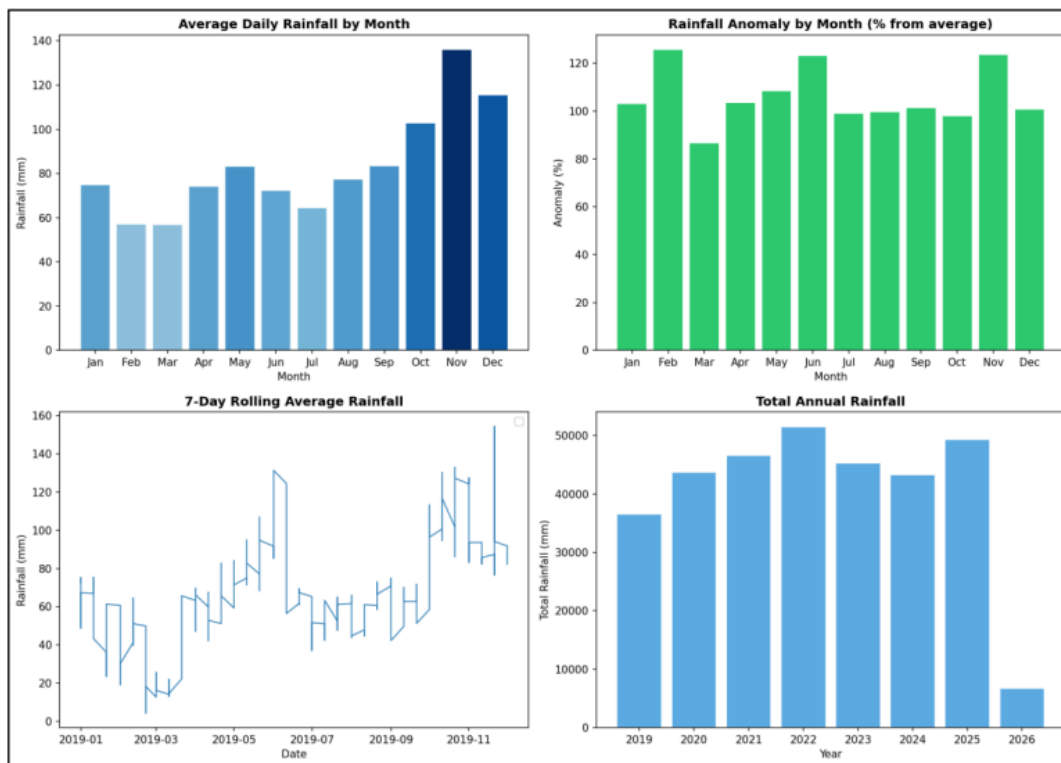
Figure 3.5 - National Rainfall Trends and Monthly Anomalies, 2019–2026
