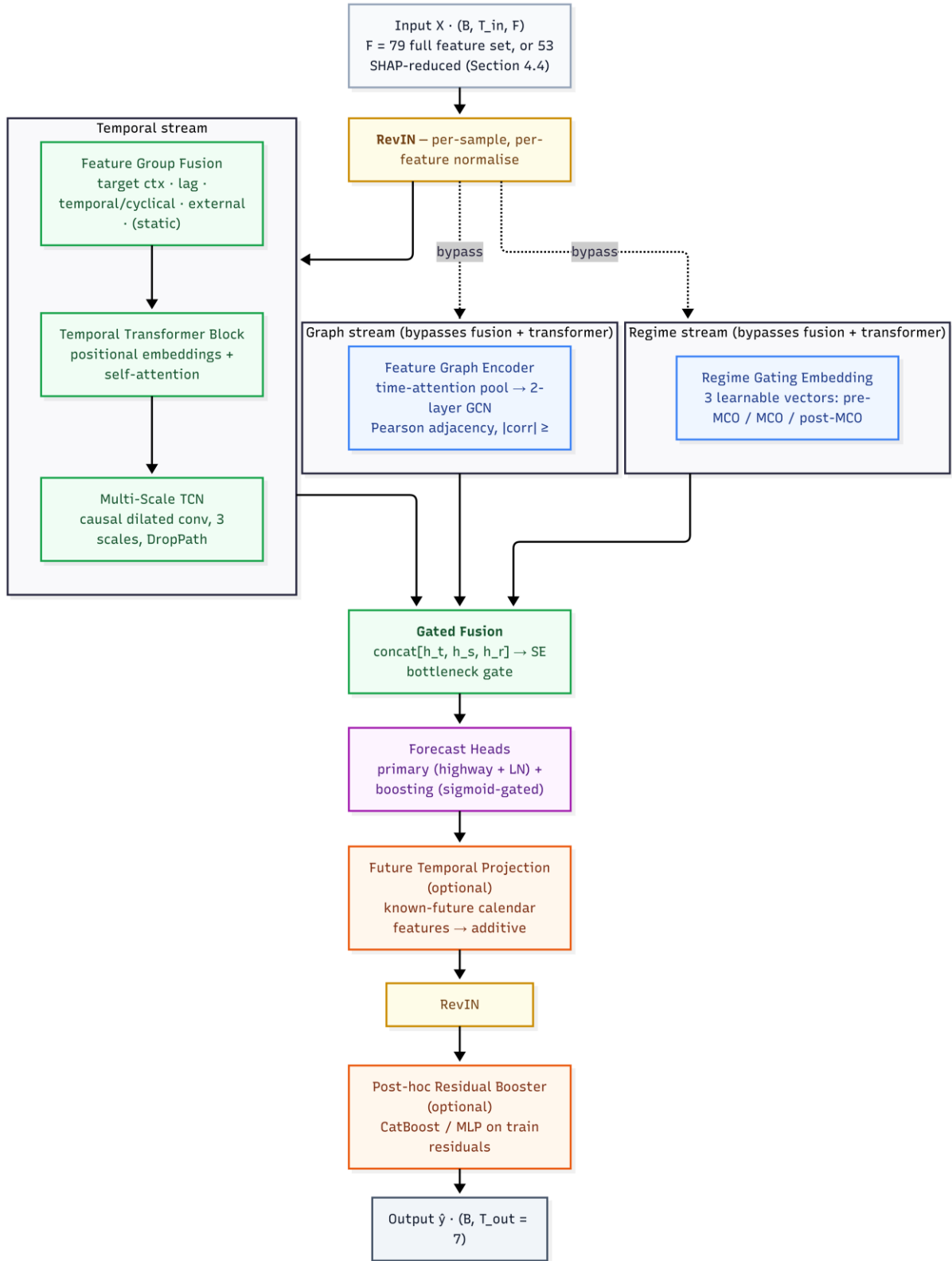
Fig. 6 Full HMT-TSF architecture, from the input tensor through RevIN and three parallel encoder streams, temporal, graph, and regime, to gated fusion, forecast heads, and denormalised output.
