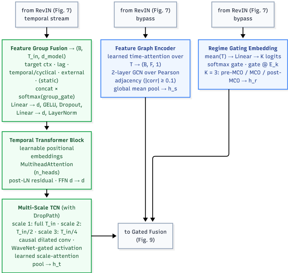
Fig. 8 Three parallel encoders: Feature Group Fusion and the Temporal Transformer Block feeding the Multi-Scale TCN ( h_t ), the Feature Graph Encoder over the Pearson adjacency ( h_s ), and the Regime Gating Embedding ( h_r ).
