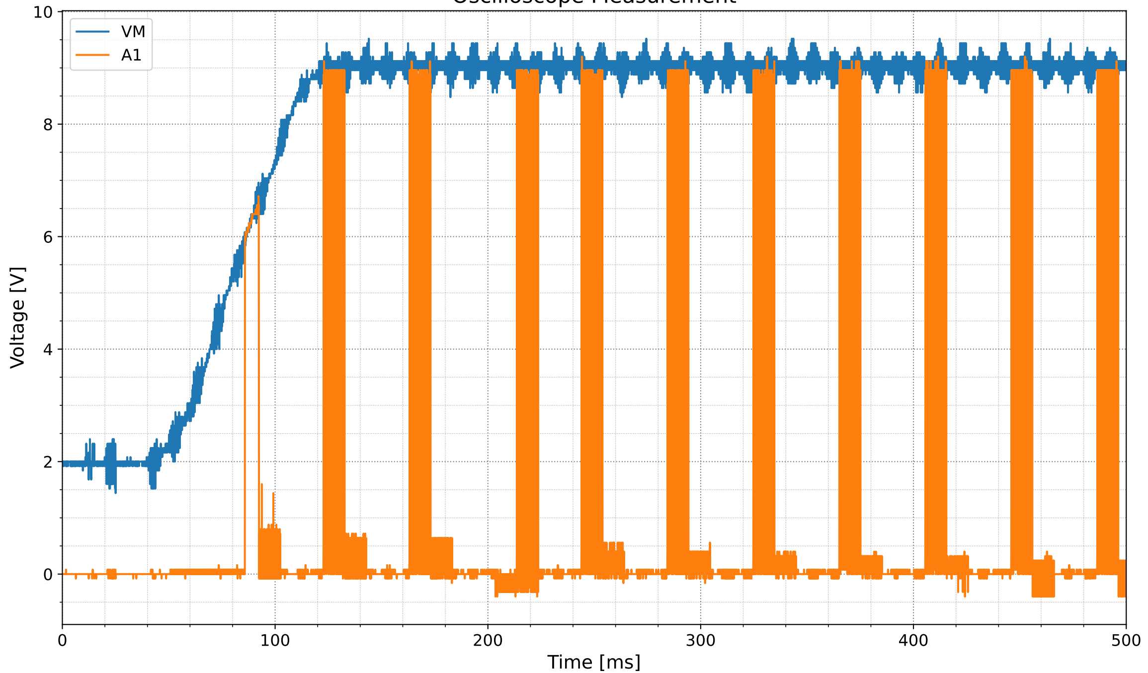
Oscilloscope Measurement
