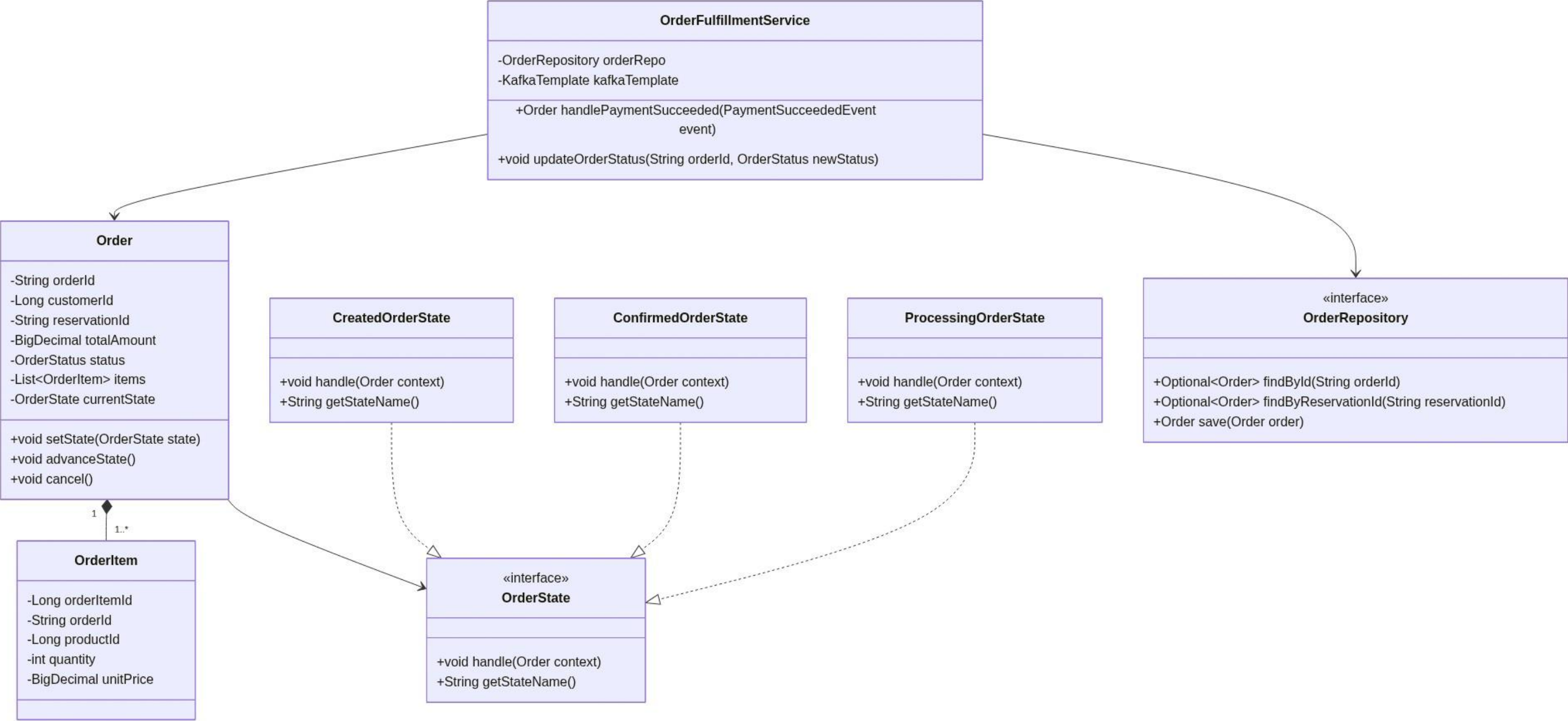
Figure: Diagram 4.3: classDiagram - Order Module
