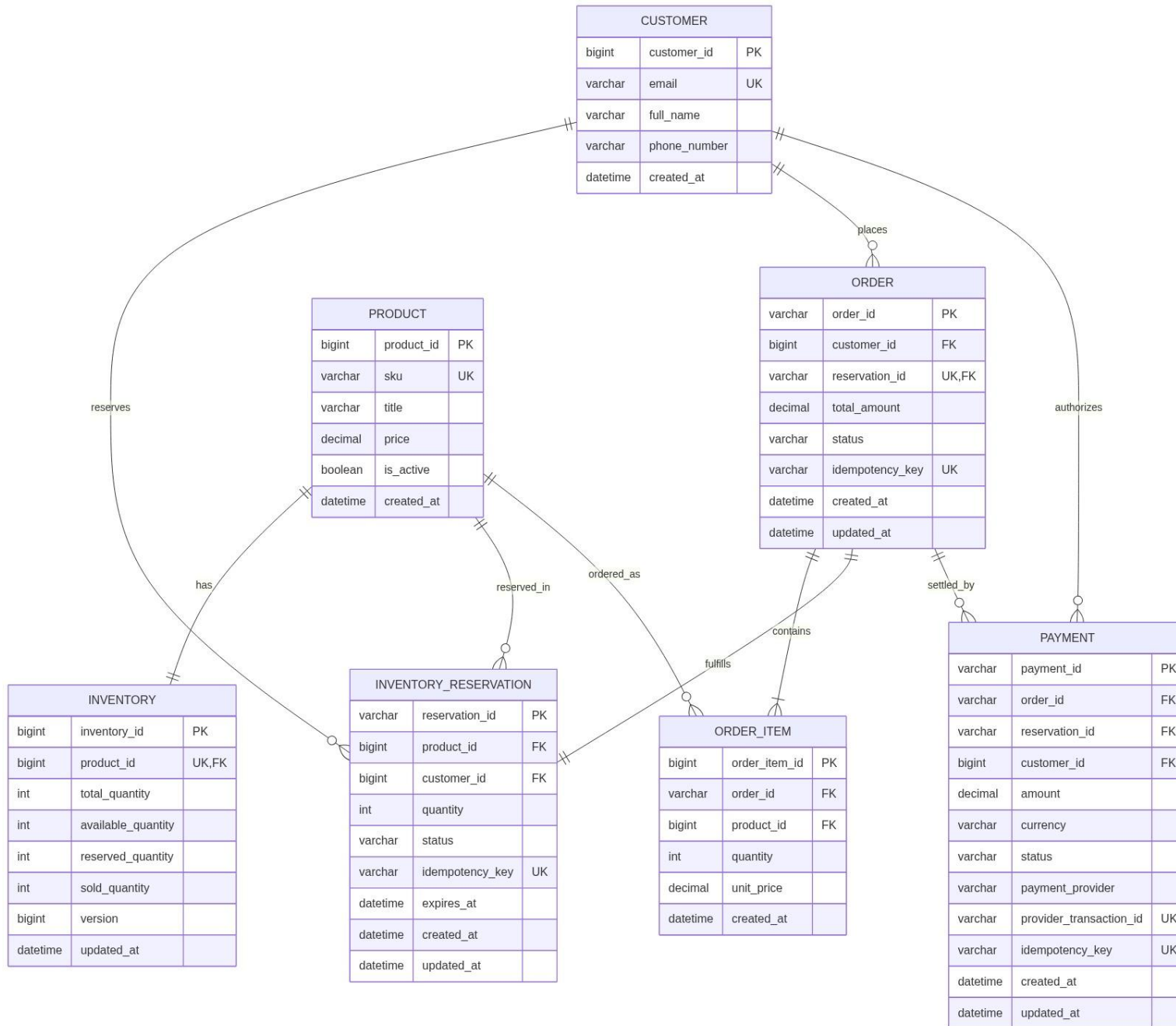
Figure: Diagram 5: erDiagram
