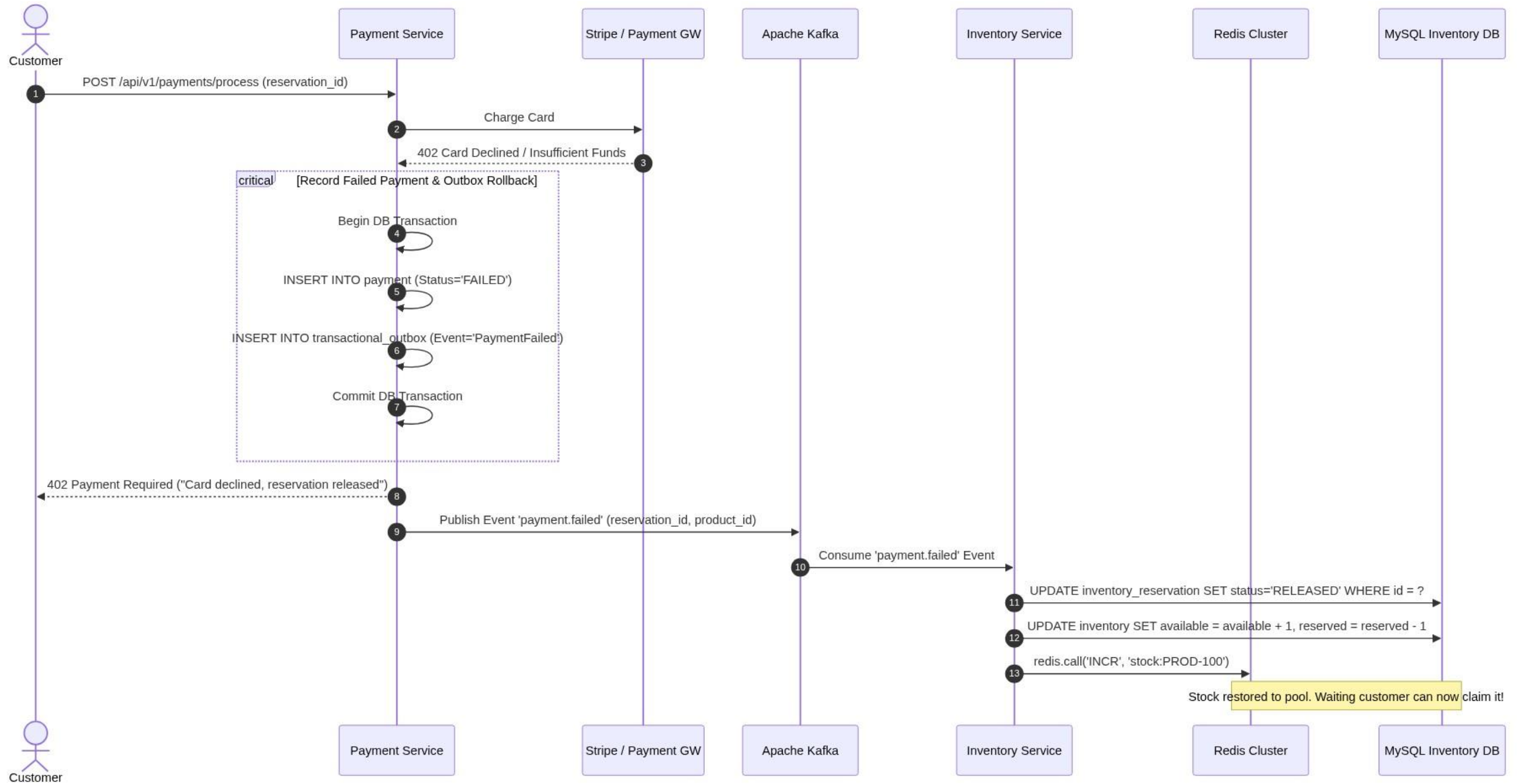
Figure: Diagram 9: sequenceDiagram
