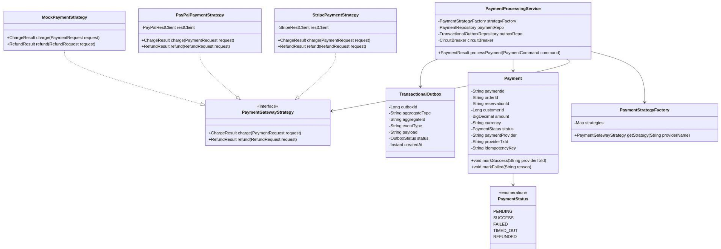
Figure: Diagram 4.2: classDiagram - Payment Module
