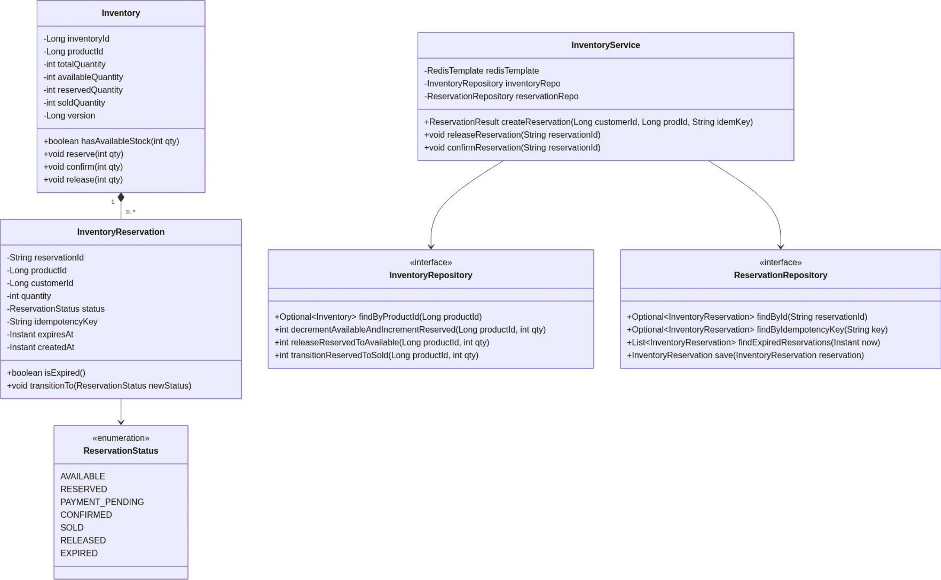
Figure: Diagram 4.1: classDiagram - Inventory Module
