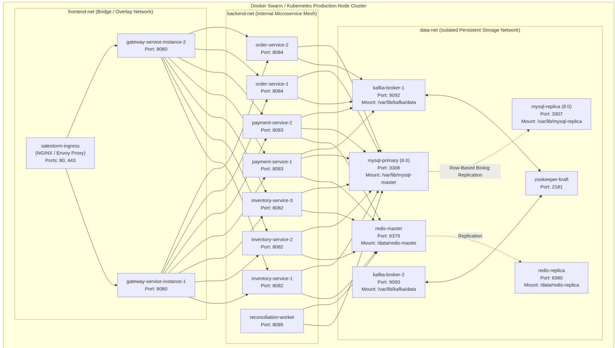
Figure: Diagram 3: flowchart TD
