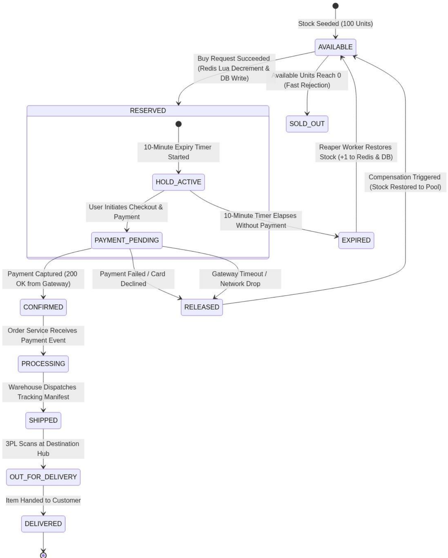
Figure: Diagram 7: stateDiagram-v2
