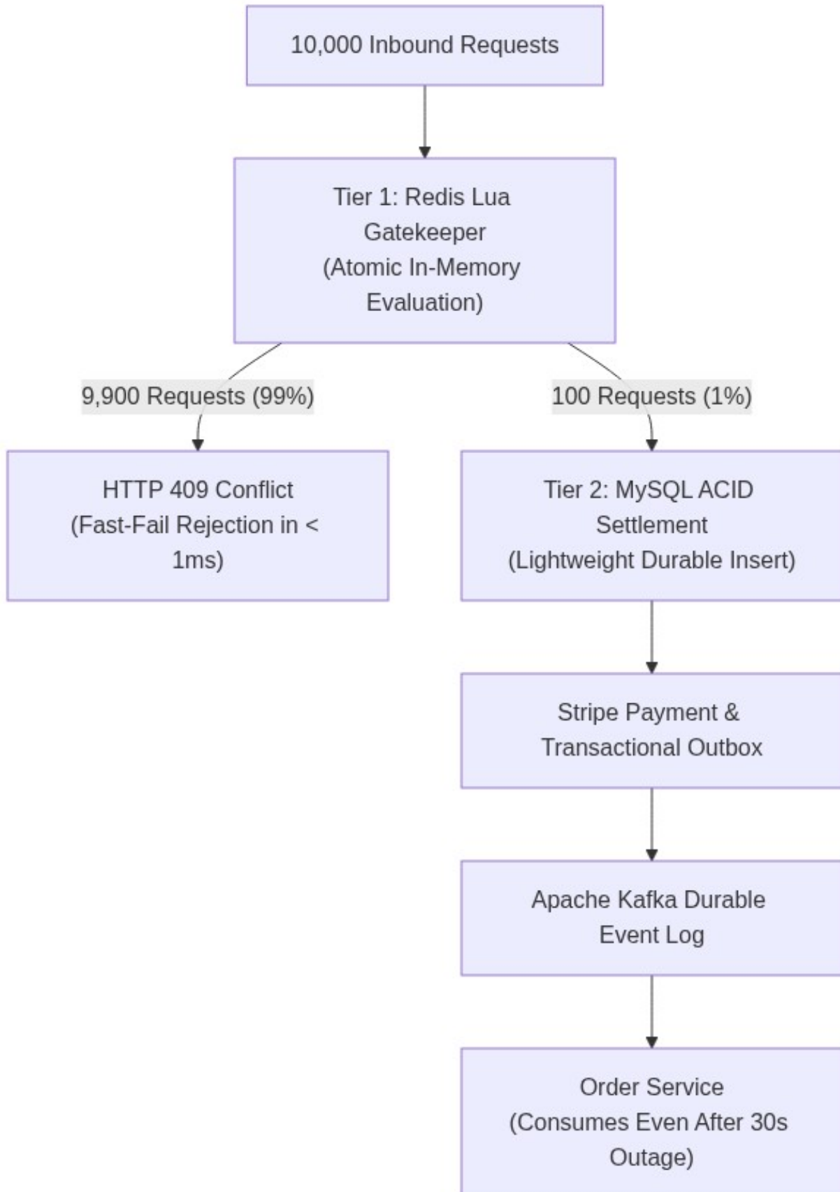
Figure: Diagram 12: flowchart TD
