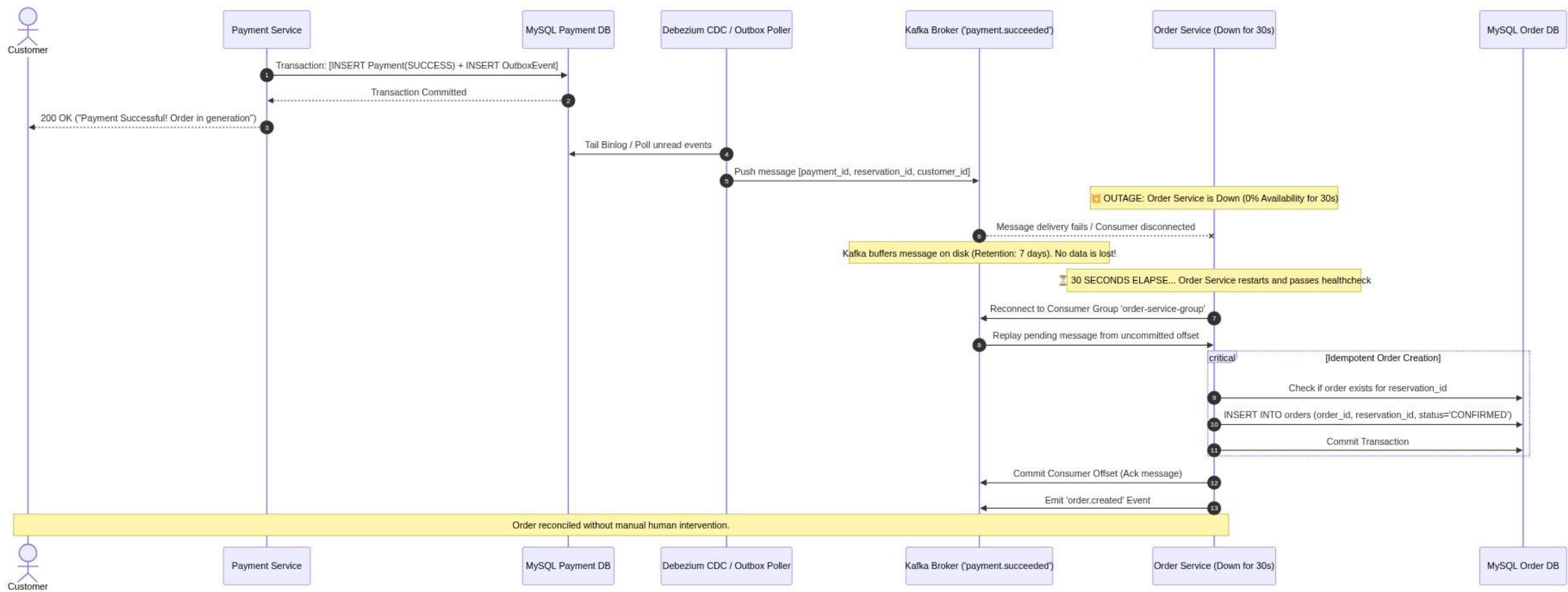
Figure: Diagram 10: sequenceDiagram
