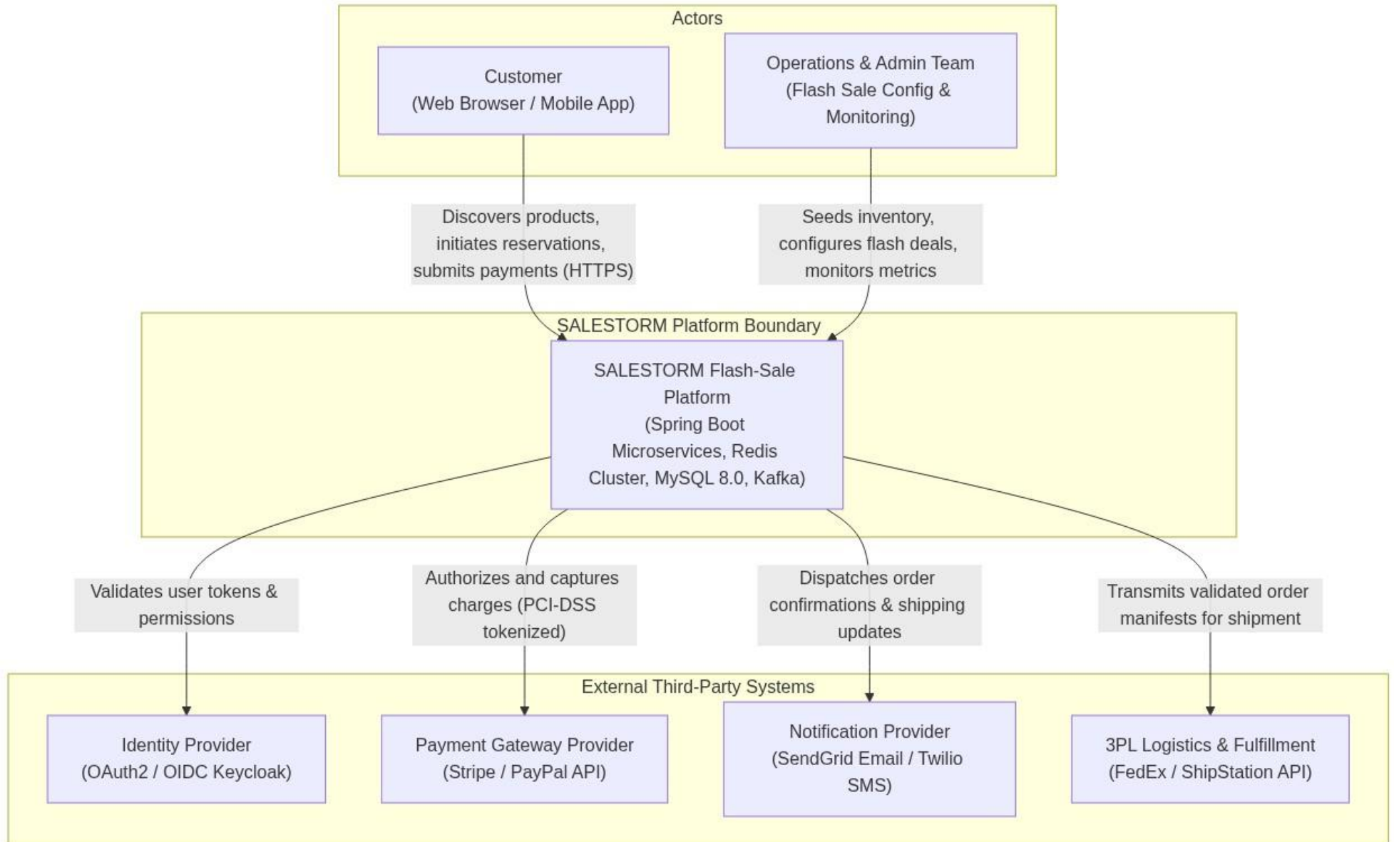
Figure: Diagram 1: flowchart TD
