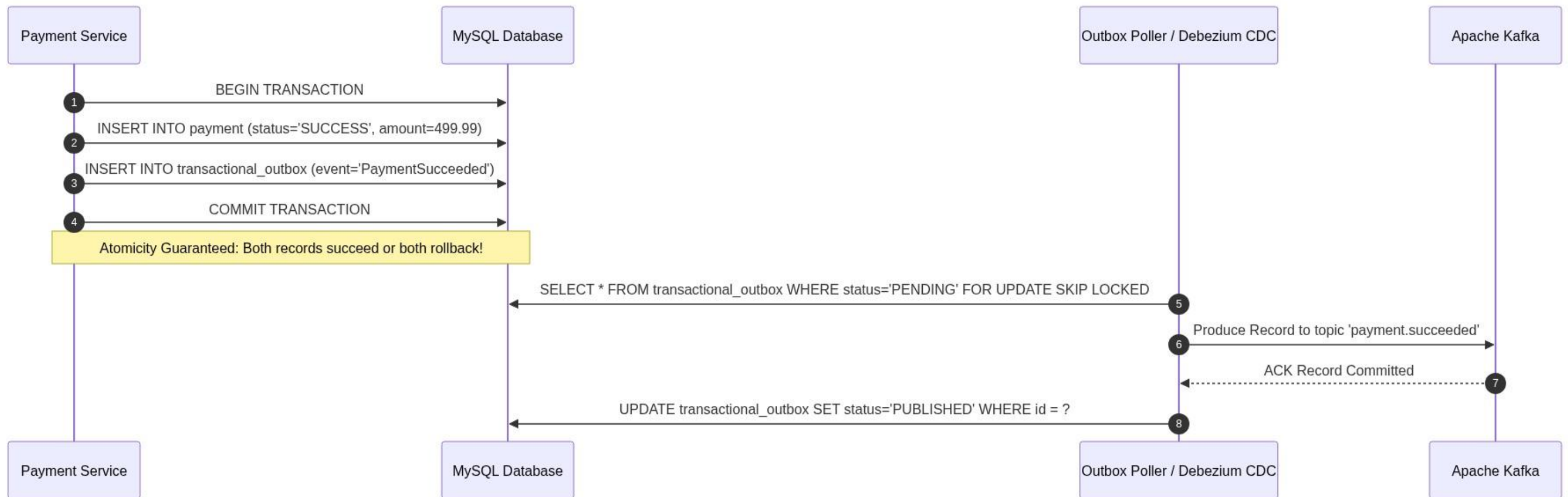
Figure: Diagram 6: sequenceDiagram
