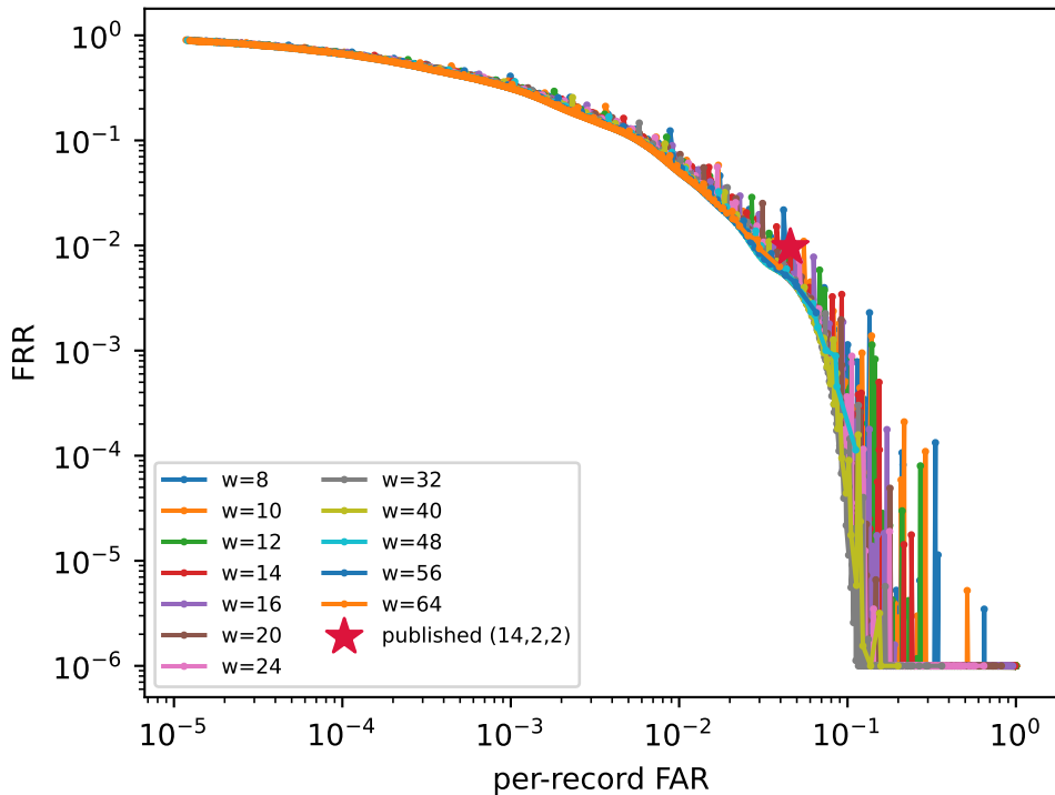
DET frontier over ( w, t, \theta )
