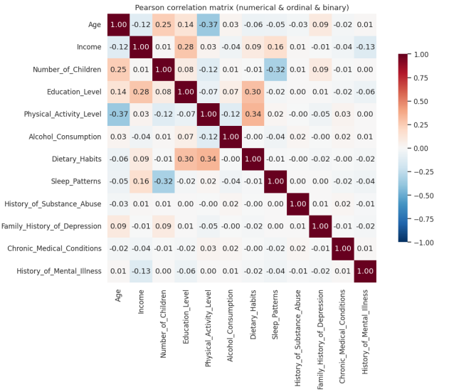
Fig. 2. Pearson correlation matrix on the numerical / ordinal / binary view. The strongest correlations are weak ( |p| < 0.40 ), notably Age \leftrightarrow Physical_Activity_Level ( p = -0.37 ) and Education_Level \leftrightarrow Dietary_Habits ( p = +0.30 ). History_of_Mental_Illness has no correlation above 0.13 with any feature.
