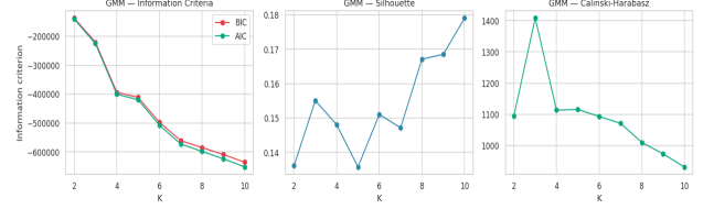
Fig. 9. GMM model selection. The information criteria are still decreasing at K = 10 , characteristic of data without a natural Gaussian cluster count.
