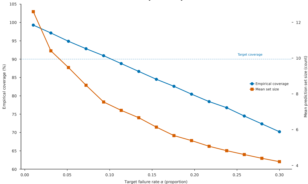
Conformal safety-efficiency trade-off
