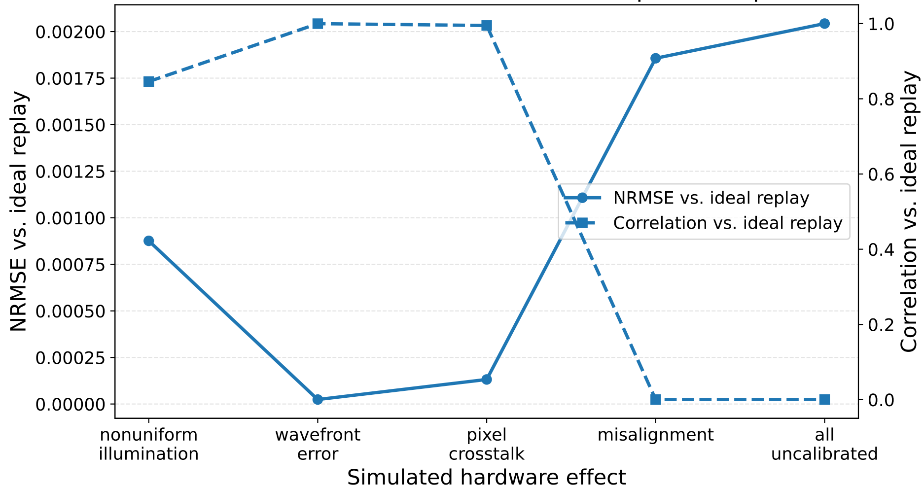
Pseudo-hardware stress test of SLM phase map
