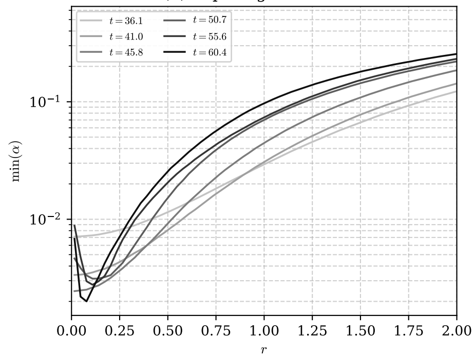
(h) Lapse against radius
