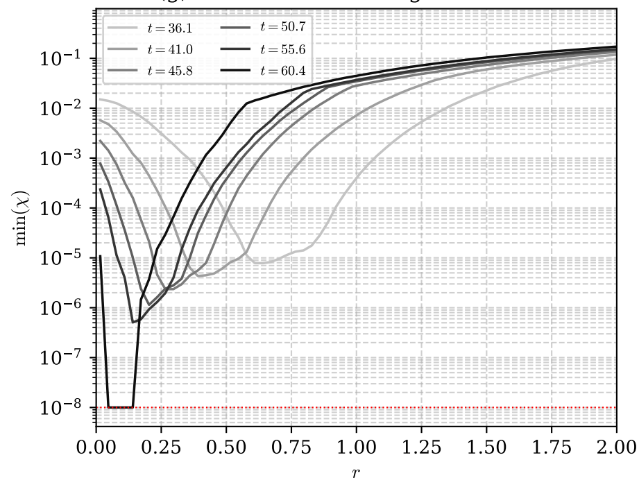
(g) Conformal factor against radius
