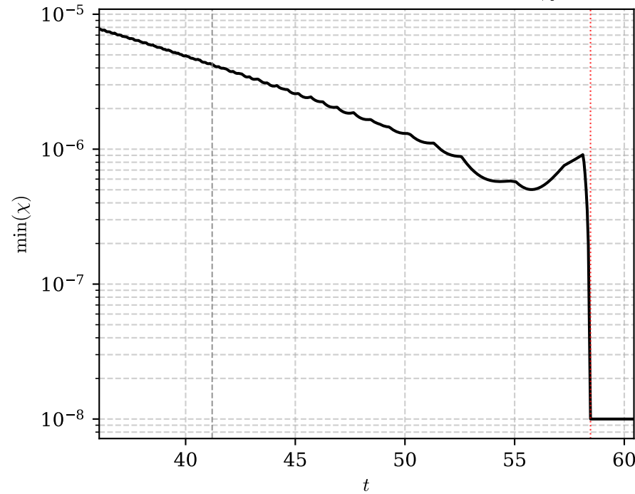
(e) Growth compared: core against constraints
