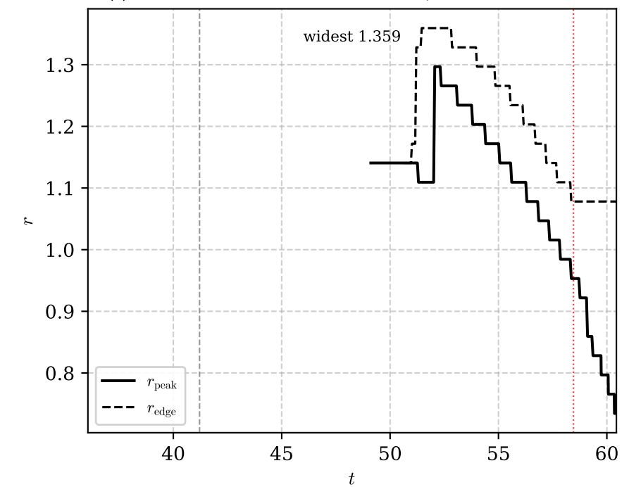
(i) Where the disturbance is, and how wide
