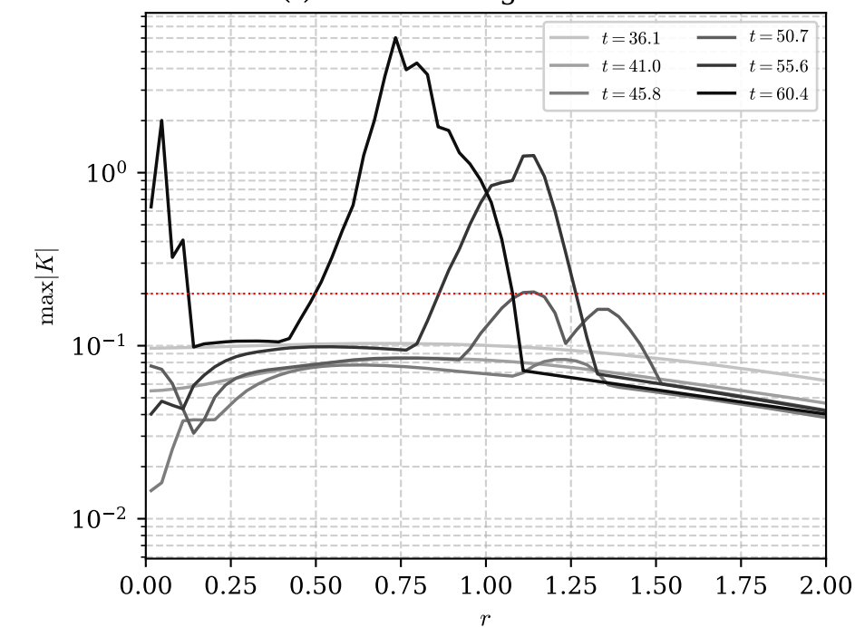
(i) Where the disturbance is, and how wide
