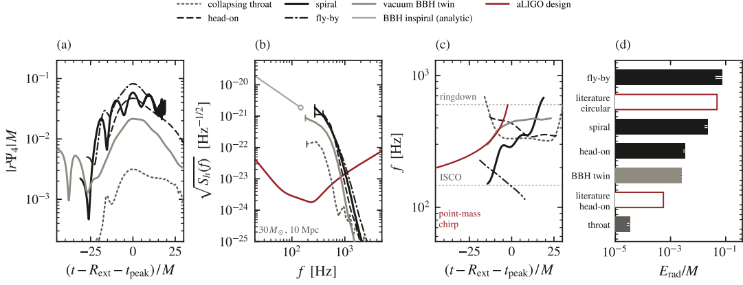
FIG. 8. Every source on a detector at one shared calibration: total mass M = 30 M_\odot , distance D = 10 Mpc, each record first reduced to units of its own total ADM mass; strain scales as M/D , frequency as 1/M . (a) Envelopes |r\Psi_4|/M at the innermost sphere on a common merger clock ( \tau = 0 at each peak): fly-by loudest ( 8.2 \times 10^{-2} ), then spiral, head-on, vacuum twin, lone throat ( 3.1 \times 10^{-3} ). (b) Strain amplitude spectral densities over the aLIGO design floor (burgundy), each curve drawn from its own low-frequency corner (one cycle per record, ticked), below which a record of length T cannot tell a wave from a drift. Read them as falling power laws (slopes -3.3 to -5.9 ) with no resolved maximum: any “peak” taken from this panel is the corner 1/T ; the values at the resolved \Psi_4 peaks are quoted in the text. Faint line: the Newtonian inspiral of the same binary, |\dot{h}| \propto f^{-7/6} to its ISCO at 147 Hz—the ramp an astrophysical binary rides into the band where the simulated signal begins. (c) Instantaneous frequency over each record’s body against the point-mass chirp (burgundy), the ISCO (147 Hz) and the equal-mass Kerr ringdown (599 Hz): the vacuum twin climbs the chirp and peaks at fM = 0.065 , the textbook merger value; no wormhole channel does (tracks in Sec. X C). (d) Energy radiated in the dominant multipole, ranked; the tick on each bar is the spread over extraction spheres, the error bar that catches near-zone content posing as a wave (fly-by 43%, the widest: the expansion of its open mouths is near-zone content the outer spheres see less of). Open burgundy bars: the published equal-mass vacuum results from rest at infinity—head-on infall 5.5 \times 10^{-4} , quasi-circular merger 4.84 \times 10^{-2} —which bracket any vacuum binary; the spiral and fly-by outradiate the vacuum twin by 8.5\times and 29\times . Energies are band integrals of |\int r\Psi_4 dt|^2 over a common retarded window, doubled for the \pm m pair; gravitational channel only—the scalar’s own energy is invisible to \Psi_4 .
