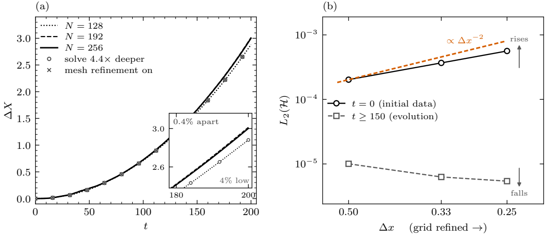
FIG. 6. (a) The resolution ladder at d_0 = 10 : midpoint drift at \Delta x = 0.50, 0.33, 0.25 , with two twins of the base rung overlaid—the elliptic solve driven 4.4 \times deeper (circles) and mesh refinement enabled (crosses); both reproduce it to 2 \times 10^{-5} . Inset: the endpoint—the two fine grids agree to 0.4% while the base rung sits 4% low. (b) Two competing error sources: the t = 0 violation rises with resolution (the solve-to-evolution transfer residual, amplified as \Delta x^{-2} ; Appendix A) while the evolution’s own falls —two opposite grid behaviours never leave a single asymptotic power.
