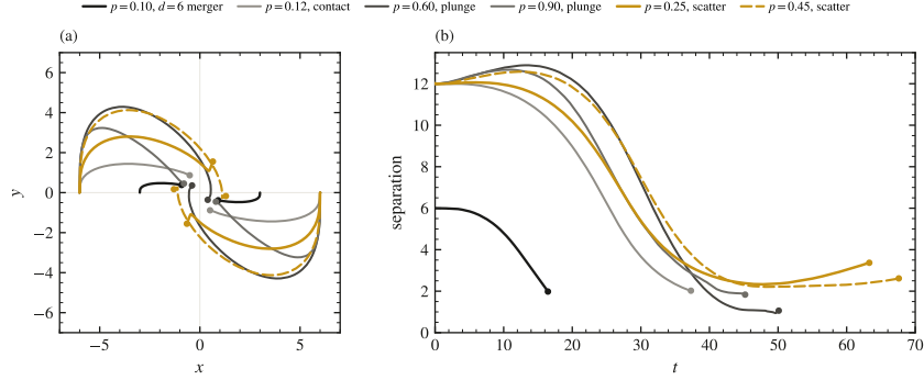
FIG. 13. Merger or fly-by on boosted, solved data: the d = 12 momentum scan and the d = 6 merger. (a) Both throats in the orbital plane; (b) their separation. The tracks are the coordinate positions of the \chi pits, followed through each run by continuity and smoothed over two time units; a track ends (dot) where its pits stop being trackable (a superluminal hop between two \chi minima) or at the run's trust window. Gold: the scatterers, p = 0.25 (solid, to t = 63.3 ) and 0.45 (dashed, to t = 67.6 ). Ink and greys: the plunges p = 0.60 and 0.90 (two legs each, concatenated across their restarts), the d = 6 , p = 0.10 merger, and the p = 0.12 arm, whose pits reach contact at t \approx 37 . Movies: Videos 8 ( p = 0.25 ) youtu.be/fh3pU7xCU_I , 9 ( p = 0.60 ) youtu.be/-ejFKpetL1Y and 10 ( p = 0.90 ) youtu.be/yzvwjC46lJY .
