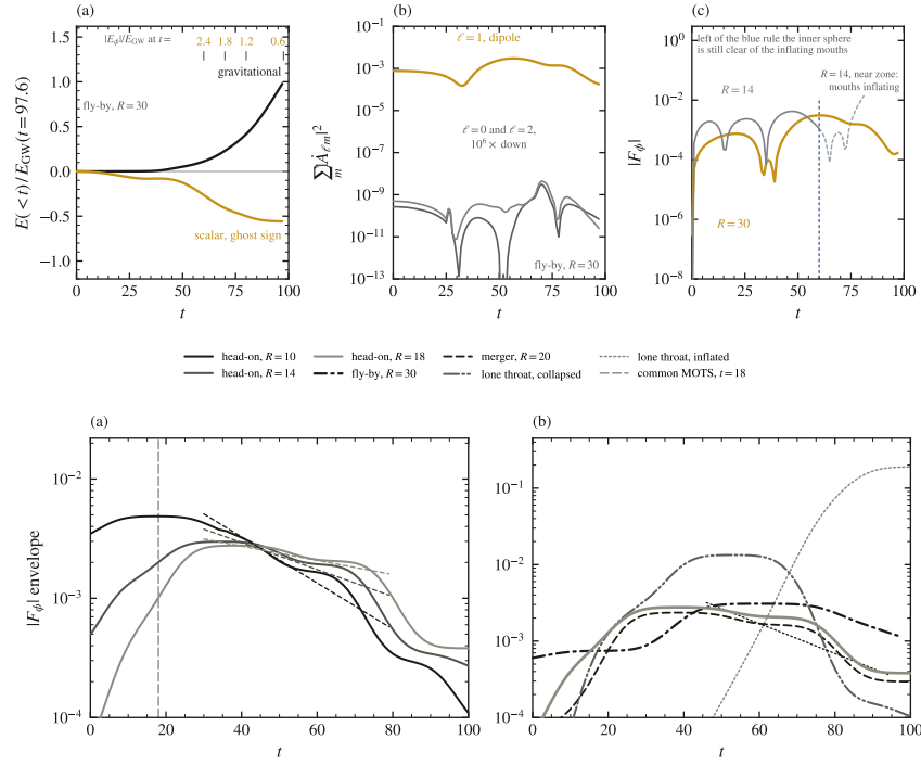
FIG. 14. Top (channel) : The scalar channel on the \Psi_4 spheres. (a) Fly-by energy through R = 30 in units of the gravitational energy crossed by the end of the sphere's trusted record ( t = 97.6 , t - R = 67.6 ): gravitational (ink) and scalar with its physical sign (gold, Sec. VIII F). The ratio |E_\phi|/E_{\text{GW}} printed at each cut falls from 2.4 at t = 60 to 0.56 over the whole record, as the gravitational burst arrives after the scalar one (Sec. VIII F). (b) Multipole content, fly-by: \ell = 1 exceeds \ell = 0 and \ell = 2 by 10^{6.4} . (c) Validity window: |F_\phi| at both spheres, each drawn to its retarded gate t - R = 67.6 . Past the blue rule ( t = 60 ) the inner sphere reads the inflating mouths' near field—its climb there has no counterpart at R = 30 one light-crossing later—so that stretch is dashed and carries no claim; the t = 60 window at R = 14 gives 0.6 in place of 2.4. Bottom (censorship) : Envelope of the scalar flux |F_\phi| , horizoned against horizonless arms: a running maximum over 25 units, smoothed in log amplitude, since the raw flux changes sign every \sim 13 units. (a) The head-on chain's glued record at R = 10/14/18 . The common MOTS closes at t = 18 (dotted); the remaining hair leaves as one \ell = 1 pulse, cresting later at each sphere, then decays (dashed: fits over t = 30-80 , \tau = 22/38/73 ). The rise before the rule is the open mouths' static hair, canonically ingoing; only the outgoing window is integrated. (b) One sphere per fate (head-on and lone throat R = 18 , merger R = 20 , fly-by R = 30 ): the merger, behind its horizon from t = 13 , decays like the head-on ( \tau = 22 , dotted fit); the fly-by, horizonless, shows its burst's complete arch, drawn to t - R = 67.6 (its trust window). Mid-grey: the lone throat twice—the \varepsilon = +10^{-2} level-4 collapse (solid), behind a MOTS from t = 11 , and the unkicked level-4 throat (dotted), which inflates, horizonless, and grows in the monopole (counted to t \approx 80 ).
