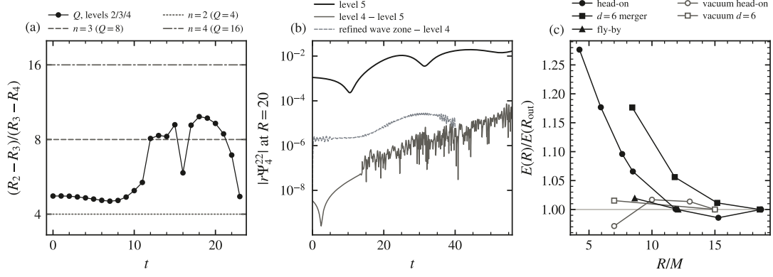
FIG. 10. Convergence. (a) The static throat from exact data at levels 2–4: the three-level factor Q = (R_2 - R_3)/(R_3 - R_4) of its minimal areal radius against the orders n = 2, 3, 4 (rules); the dip at t = 16 is one level-2 dump. (b) |r\Psi_4^{22}| at R = 20 of the d = 12, p = 0.12 pair with Bowen–York momentum (otherwise our data) at throat level 5, its difference from level 4, and the difference made by refining the wave zone to half the base cell. (c) Radiated energy on each sphere over the outermost sphere’s, against R/M : the head-on, the d = 6 merger and the fly-by (ink) and two vacuum controls (grey). The outcome: the scheme converges at order 3.0–3.3, a binary’s waveform is resolved to 0.4% of its peak, and the energy converges in extraction radius.
