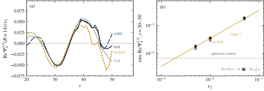
FIG. 12. Linearity of the collapsing throat's wave in its quadrupole seed. (a) \text{Re } \Psi_4^{2,0} at R = 14 , each arm divided by its seed and named at its end: \varepsilon_2 = 0.005, 0.01, 0.05 and the kick-free 0.01 arm collapse onto one curve through the burst; later the smallest arm carries its floor amplified by 1/\varepsilon_2 and the kick-free arm runs ahead. (b) rms amplitude over t = 30\text{--}50 against \varepsilon_2 at three spheres, with the slope-one line through the 0.01 arm drawn across the decade 10^{-3}\text{--}10^{-1} as a reference. Open circle: the pure quadrupole, within 2% of the kicked arm. Dashed rule: the floor of the level-4 spherical control (the same kick, no quadrupole) at R = 14 , which the line crosses at \varepsilon_2 \approx 2 \times 10^{-3} . The outcome: the wave is the quadrupole's—linear in \varepsilon_2 and unchanged, to 2% in amplitude, when the radial kick is removed. The kick alone radiates only the floor; it moves the wave's phase, not its size.
