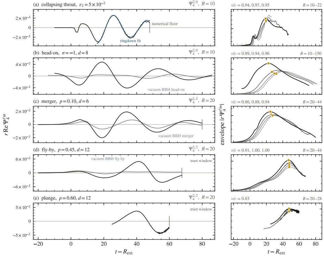
FIG. 8. The waveform gallery: one row per scenario on one retarded clock. Left: r \operatorname{Re} \Psi_4 of the dominant mode at the innermost sphere, each row on its own scale; row (a) is the \varepsilon_2 = 0.05 arm, with the ringdown fit of Sec. VIII A dashed (period 20.6 M ). Caps mark where the drawn record ends: the collapsing throat before its numerical floor exceeds 14% of the burst peak; the fly-by at its trust window ( t - R = 67.6 ), the plunge at its own. Row (b) is the same head-on rerun in an L = 512 box with spheres to R = 150 , clean to the clock's edge. The merger runs through remnant ringdown, with one linear bridge across a leg seam. Grey under (b)–(d): the vacuum controls, black holes at the same d and p on bare punctures, on the same scale: the vacuum head-on rings 5.4\times lower and crests later (Sec. VIII B); the vacuum merger peaks at the drainhole merger's retarded time, 3.0\times lower; the vacuum fly-by radiates one cycle as the holes swing away from periapsis, 6.7\times below the fly-by's arch. Right: the amplitude envelope at every sphere on its own retarded time (ink to faint, inner to outer)—the upper envelope of |r \Psi_4| for the complex (2, 2) modes, the analytic-signal envelope for the real (2, 0) modes—which folds onto one curve for a signal moving at c and falling as 1/r . Gold dots: the correlated wavefront. The quoted v/c is the whole-waveform lag between neighbouring spheres (Sec. VIII E), the plunge's the burst-peak lag: throat 0.94/0.97/0.95, head-on 0.89/0.94/0.96, merger 0.86/0.88/0.94, fly-by 0.91/1.00/1.00, plunge 0.83. Movies of the far-zone head-on, whose remnant spreads with the coordinates while its area holds, and of the vacuum head-on and fly-by: Videos 11 youtu.be/vesOxaP5GSg , 8 youtu.be/aRWvD4W8OOg and 9 youtu.be/65_3kw4obvE .
