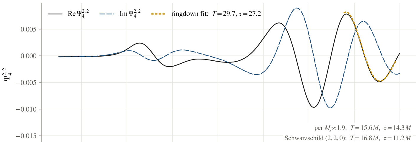
(a) the (2, 2) mode at R = 30 , BBH control to t = 150
