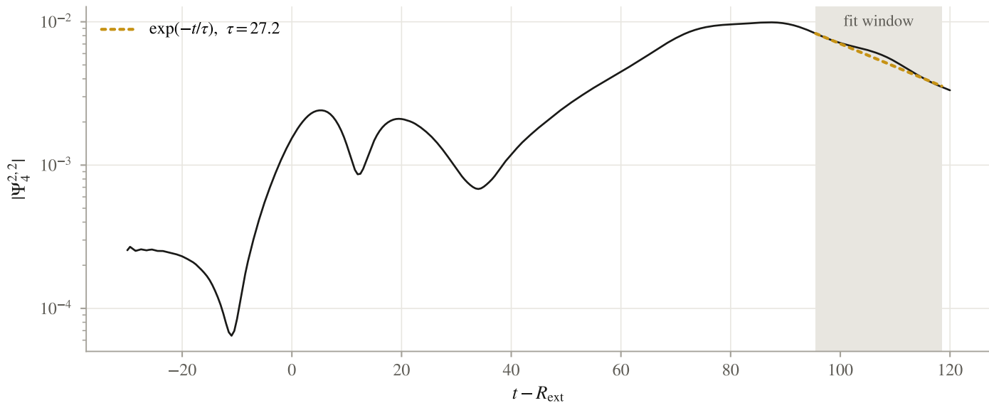
(b) envelope and the fitted exponential decay
