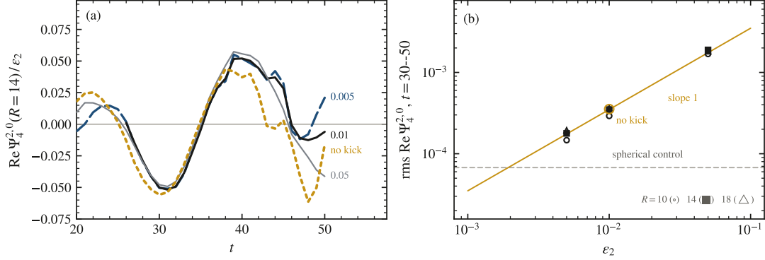
FIG. 11. Linearity of the collapsing throat's wave in its quadrupole seed. (a) \text{Re } \Psi_4^{2,0} at R = 14 , each arm divided by its seed and named at its end: \varepsilon_2 = 0.005, 0.01, 0.05 and the kick-free 0.01 arm collapse onto one curve through the burst; later the smallest arm carries its floor amplified by 1/\varepsilon_2 and the kick-free arm runs ahead. (b) rms amplitude over t = 30-50 against \varepsilon_2 at three spheres, with the slope-one line through the 0.01 arm drawn across the decade 10^{-3}-10^{-1} as a reference. Open circle: the pure quadrupole, within 2% of the kicked arm. Dashed rule: the floor of the level-4 spherical control (the same kick, no quadrupole) at R = 14 , which the line crosses at \varepsilon_2 \approx 2 \times 10^{-3} . The outcome: the wave is the quadrupole's—linear in \varepsilon_2 and unchanged, to 2% in amplitude, when the radial kick is removed. The kick alone radiates only the floor; it moves the wave's phase, not its size.
