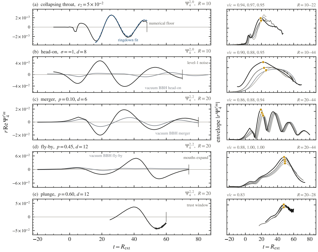
FIG. 7. The waveform gallery: one row per scenario on one retarded clock. Left: r \text{Re } \Psi_4 of the dominant mode at the innermost sphere, each row on its own scale; row (a) is the \varepsilon_2 = 0.05 arm, with the ringdown fit of Sec. VIII A dashed (period 20.6 M ). Caps mark where the drawn record ends: the collapsing throat where its numerical floor passes 10% of the burst peak; the head-on where the noise of its level-1 refinement cube reaches the sphere (from t = 80 at R \leq 20 ); the fly-by at the trough where the mouths' expansion meets the decaying arch ( t - R = 74 ); the plunge at its trust window. The merger runs whole, burst through remnant ringdown. Grey under (b)–(d): the vacuum controls, black holes at the same d and p on bare punctures, on the same scale: the vacuum head-on rings 6.1 \times lower and crests later (Sec. VIII B); the vacuum merger peaks at the drainhole merger's retarded time, 3.0 \times lower; the vacuum fly-by radiates one cycle as the holes swing away from periapsis, 6.7 \times below the fly-by's arch. Right: the amplitude envelope at every sphere on its own retarded time (ink to faint, inner to outer)— |r \Psi_4| for the complex (2, 2) modes, the analytic-signal envelope for the real (2, 0) modes—which folds onto one curve for a signal moving at c and falling as 1/r . Gold dots: the correlated wavefront. The quoted v/c is the whole-waveform lag between neighbouring spheres (Sec. VIII E), the plunge's the burst-peak lag: throat 0.94/0.97/0.95, head-on 0.94/0.88/0.95, merger 0.86/0.88/0.94, fly-by 0.88/1.00/1.00, plunge 0.83. Movies of the vacuum head-on and fly-by: Videos 5 youtu.be/aRWvD4W8OOg and 6 youtu.be/65_3kw4obvE .
