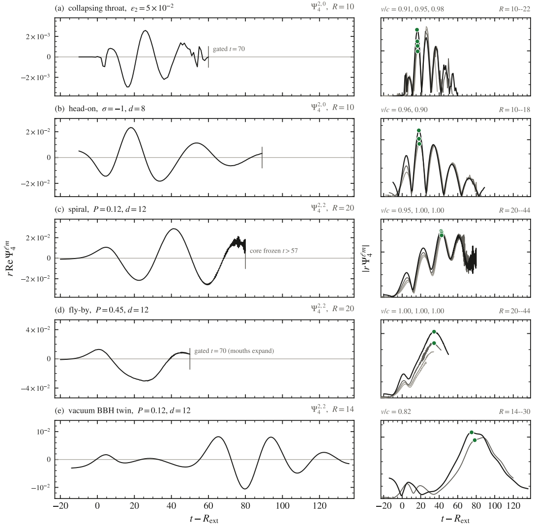
FIG. 8. The waveform gallery: every channel’s radiation, one row per scenario, one retarded clock. Left column: r \text{Re} \Psi_4 of the dominant mode at the innermost extraction sphere, each row on its own stated scale—the lone throat radiates an order of magnitude below the mergers, and the fly-by is the loudest channel of all. Half-height caps mark record ends: the collapsing throat’s stream is junk-gated at t = 70 , the spiral is drawn to t = 60 —the end of its no-fill profiled leg, past which the record continues only behind a core frozen at t = 57 (Sec. VII C), so the panel stops where the interior is still evolved—and the fly-by—complete to t = 100 , no horizon ever forming—is gated at t = 70 , ahead of the t = 76.1 trough where the mouths’ expansion (areal radii growing \times 7.8 ) has grown to equal the decaying burst at the R = 20 sphere. Right column: the envelope |r \Psi_4| at every extraction sphere on its own retarded time (ink to faint, inner to outer): a signal travelling at c and falling as 1/r folds onto one curve. Green dots mark the correlated wavefront, and the quoted v/c is the lag of the whole complex waveform between neighbouring spheres over their common retarded window—peak-to-peak timing fails on flat-topped envelopes (the vacuum twin’s merger plateau is \sim 15 units wide at both spheres, and its peak times alone would read v = 0.57c where the waveform lag reads 0.82c ). Measured speeds: throat 0.91/0.95/0.98 , head-on 0.96/0.90 , spiral 0.95/1.00/1.00 , fly-by 1.00/1.00/1.00 , vacuum twin 0.82 . Every channel propagates at c within the output cadence: radiation, not a gauge or constraint mode.
