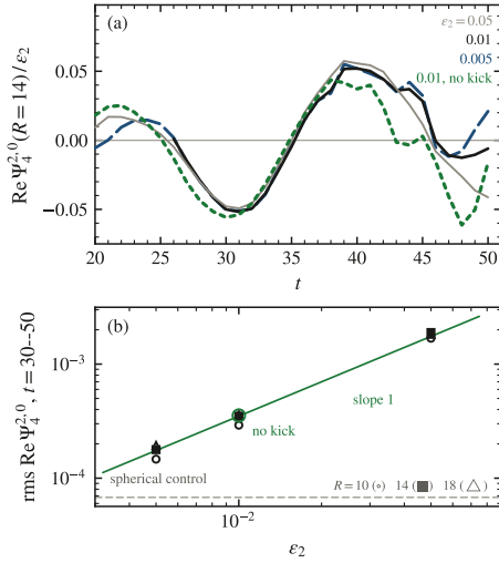
FIG. 10. One throat’s wave is linear in its deformation. (a) \text{Re } \Psi_4^{2,0} at R = 14 , each arm divided by its own seed: \epsilon_2 = 0.005, 0.01, 0.05 and the kick-free 0.01 arm collapse onto one curve. (b) rms amplitude over t = 30-50 against \epsilon_2 at three spheres, with the slope-one line through the 0.01 arm: linear to 1–16% across a decade. The open circle is the pure quadrupole—no radial kick—matching the kicked arm to 2–3%; the dashed rule is the spherical control’s floor.
