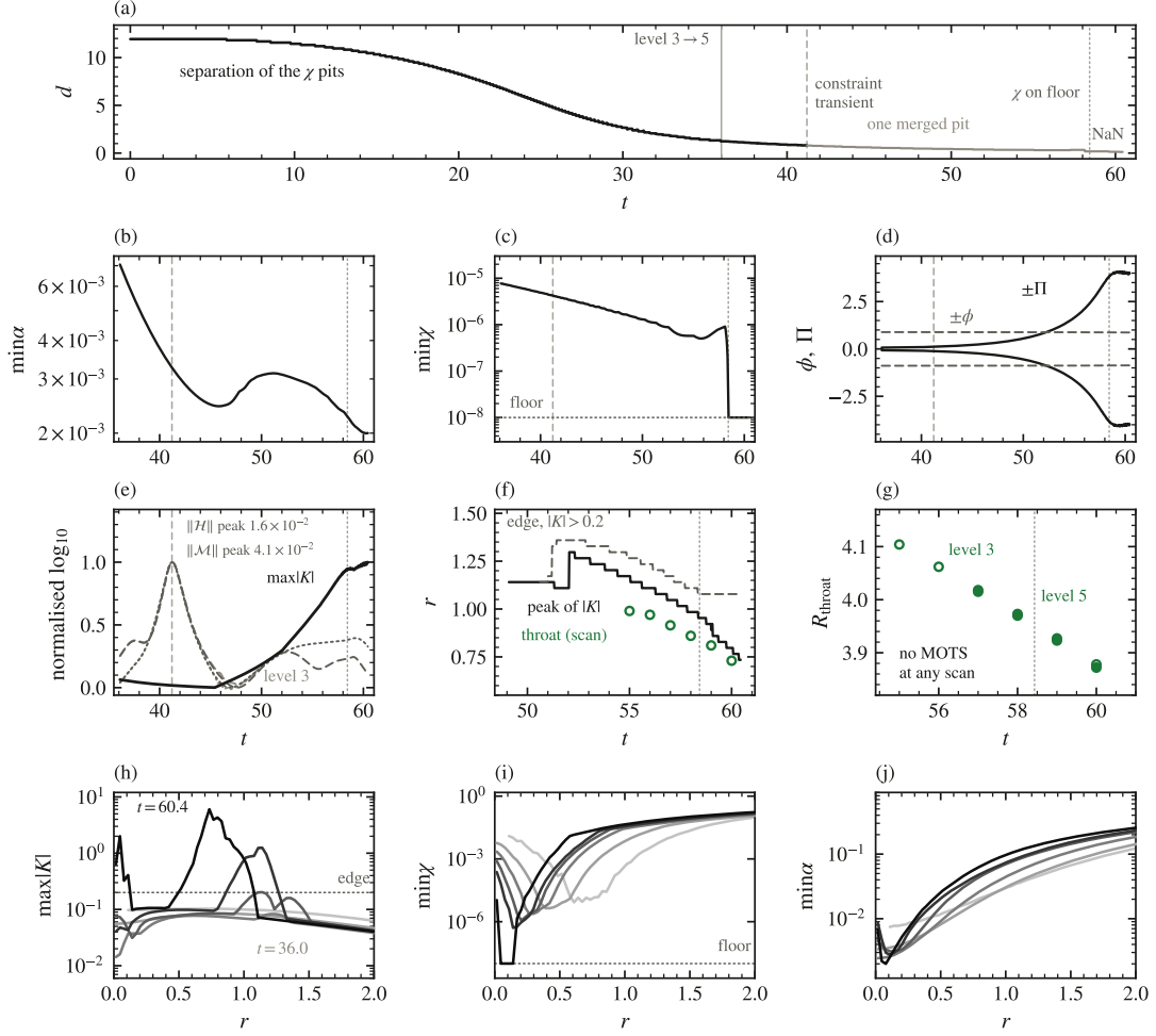
FIG. 6. The production spiral's collapse ( p = 0.12 , d = 12 ): level 5 from the restart at t = 36 to the death by NaN at t = 60.44 , no panel involving the interior fill. Rules in every time panel: the handover at t = 36 (solid), the merger transient at t = 41.2 (dashed), the \chi floor at t = 58.43 (dotted). (a) Separation of the two \chi pits over the whole history—the level-3 leg carries the plunge from d = 11.9 , after which the tracker follows one merged pit (pale). (b)–(d) \min \alpha bottoms at 2.0 \times 10^{-3} without reaching zero; \min \chi decays exponentially onto its 10^{-8} floor at r = 0.078 ; the scalar holds \pm 0.89 while \Pi saturates at \pm 4.1 —the profile survives, the momentum diverges. (e) Growth compared, each curve \log_{10} -scaled onto [0, 1] : the constraint norms peak at the merger and relax below where they started, while \max |K| climbs only from t = 49 , with \text{corr}(\log \max |K|, \log \|\mathcal{H}\|) = -0.35 after t = 40 —the death is not a constraint blow-up. Pale: the level-3 leg through the same transforms, median 3.5% ( \mathcal{H} ) and 0.7% ( \mathcal{M} ) over t = 36 –50. (f) Radius of the |K| spike (steps, drawn from t = 49.1 ; earlier the profile is flat and an argmax is noise) and the |K| > 0.2 edge (dashed), widest at r = 1.36 . Green: the throat radius from the corrected scans—the spike rides just outside the throat and lands on it by the death. (g) Throat areal radius 4.10 \rightarrow 3.87 over t = 55 –60, levels 3 and 5 agreeing to 0.2%, with no marginally outer-trapped surface at any scan. (The in-code \theta_+ columns are omitted: their naive +r orientation manufactures trapped verdicts near a throat.) (h)–(j) Radial anatomy at six equally spaced times, light ( t = 36.1 ) to dark ( t = 60.4 ): per-shell \max |K| grows 0.08 \rightarrow 6.1 on a spike \sim 0.25 wide migrating inward, while the \chi and lapse pits stay at r \lesssim 0.15 —the gauge collapse and the curvature wall are different places.
