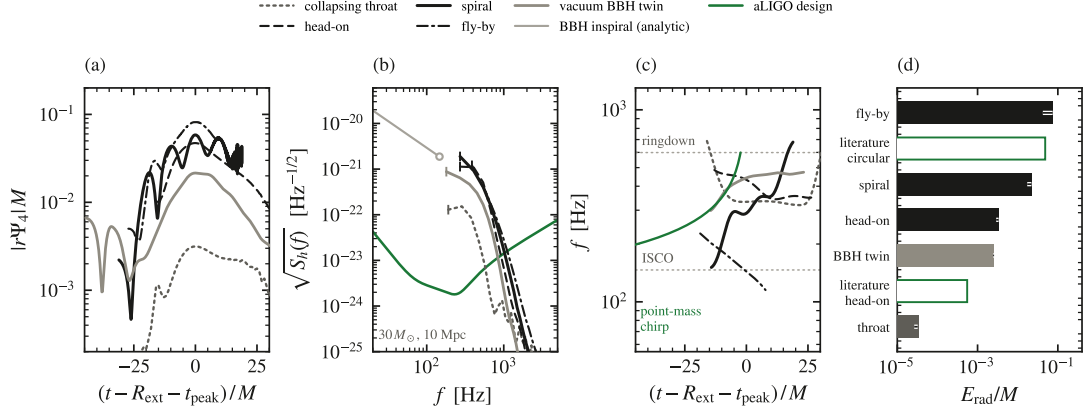
FIG. 9. Every source on a detector at one shared calibration: total mass M = 30 M_\odot , distance D = 10 Mpc, each record first reduced to units of its own total ADM mass; strain scales as M/D , frequency as 1/M . (a) Envelopes |r\Psi_4|/M at the innermost sphere on a common merger clock ( \tau = 0 at each peak): fly-by loudest ( 8.2 \times 10^{-2} ), then spiral, head-on, vacuum twin, lone throat ( 3.1 \times 10^{-3} ). (b) Strain amplitude spectral densities over the aLIGO design floor (green), each curve drawn from its own low-frequency corner (one cycle per record, ticked), below which a record of length T cannot tell a wave from a drift. Read them as falling power laws (slopes -3.3 to -5.9 ) with no resolved maximum: any “peak” taken from this panel is the corner 1/T ; the values at the resolved \Psi_4 peaks are quoted in the text. Faint line: the Newtonian inspiral of the same binary, |\tilde{h}| \propto f^{-7/6} to its ISCO at 147 Hz—the ramp an astrophysical binary rides into the band where the simulated signal begins. (c) Instantaneous frequency over each record’s body against the point-mass chirp (green), the ISCO (147 Hz) and the equal-mass Kerr ringdown (599 Hz): the vacuum twin climbs the chirp and peaks at fM = 0.065 , the textbook merger value; no wormhole channel does (tracks in Sec. XC). (d) Energy radiated in the dominant multipole, ranked; the tick on each bar is the spread over extraction spheres, the error bar that catches near-zone content posing as a wave (fly-by 43%, the widest: the expansion of its open mouths is near-zone content the outer spheres see less of). Open green bars: the published equal-mass vacuum results from rest at infinity—head-on infall 5.5 \times 10^{-4} , quasi-circular merger 4.84 \times 10^{-2} —which bracket any vacuum binary and need not bracket a ghost one; the spiral and fly-by outradiate the vacuum control by 8.5\times and 29\times , the latter against a control matched to the spiral’s momentum rather than the fly-by’s. Energies are band integrals of |\int r\Psi_4 dt'|^2 over a common retarded window, doubled for the \pm m pair; gravitational channel only—the scalar’s own energy is invisible to \Psi_4 and is measured separately in Sec. VIIF, where it is larger than every bar here and of the opposite sign.
