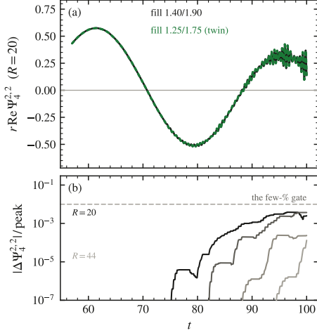
FIG. 11. Moving the fill window does not move the wave. (a) r \text{Re } \Psi_4^{2,2} at R = 20 for the freeze arm (fill 1.40/1.90, ink) and its twin (1.25/1.75, green dots), same t = 57 checkpoint, same binary: one bicolour curve. (b) The per-sphere envelope of the difference against the few-percent gate: at most 0.385% of peak at R = 20 and 0.013% at R = 44 , each front arriving on the fill’s causal clock t = 57 + (R - 1.9) . The figure certifies the fill’s inertness, not a remnant ringdown.
