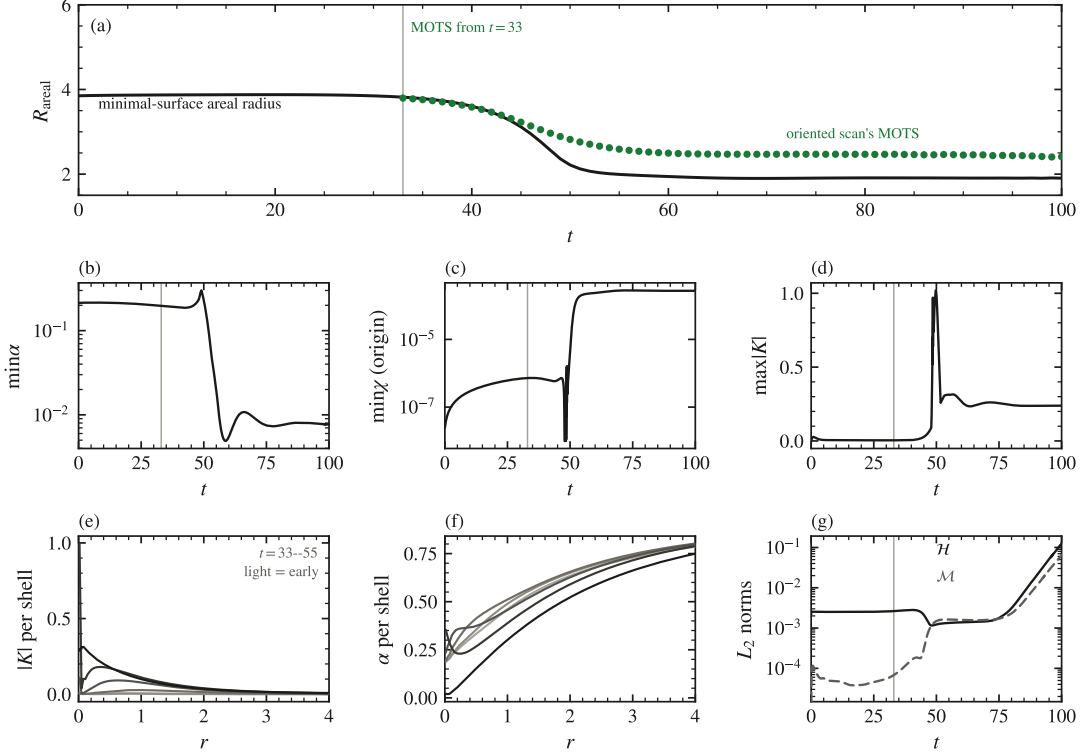
FIG. 2. The pure quadrupole’s collapse, fully instrumented (‘no kick’ arm: \varepsilon_2 = 0.01 , radial kick zero). (a) Minimal-surface areal radius (ink) and the oriented scan’s MOTS (green) from t = 33 : R falls 3.80 \rightarrow 2.41 and M_{\text{MS}} 1.90 \rightarrow 1.24 —phantom infall removes mass. (b)–(d) Global \min \alpha , \min \chi (the origin monitor, the far sheet’s compactified infinity) and \max |K| ; the violent phase is t = 45 – 55 . (e)–(f) The radial profile’s 128 shells over t = 33 – 55 (light = early): |K| grows inward while \alpha pinches to zero at the centre. (g) Constraint norms; the late rise from t \gtrsim 75 is this family’s known sphere-local floor growth, shared with the unkicked control.
