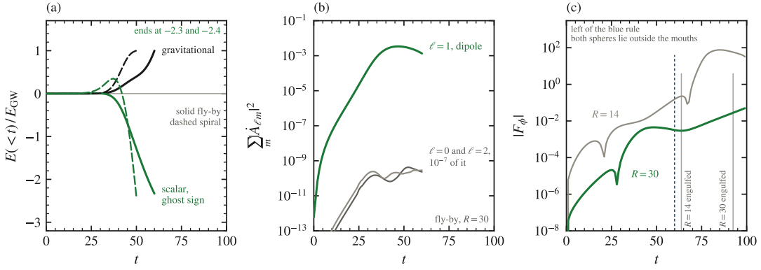
FIG. 12. The second radiation channel, on the same extraction spheres as \Psi_4 . (a) Energy through R = 30 against time, each arm in units of its own gravitational-wave energy at the rule: the gravitational curve rises to 1 by construction, the scalar curve falls to -2.3 (fly-by, solid) and -2.4 (spiral, dashed). The scalar energy is negative because gravity couples to minus this field’s stress tensor, so an outgoing scalar wave carries negative energy and the bound system gains. (b) Which multipole carries it: \ell = 1 against \ell = 0 and \ell = 2 for the fly-by, the dipole a factor 10^7 above both. Two opposite scalar charges radiate at dipole order; a vacuum binary has no such channel. (c) Where the instrument stops: |F_\phi| at both spheres against the times at which the inflating mouths’ areal radius passes each sphere’s own radius (grey rules). Left of the blue rule both spheres lie outside the mouths, and the energies in (a) are taken there; the same window read at R = 14 gives 3.0 in place of 2.3, which is this measurement’s error bar.
