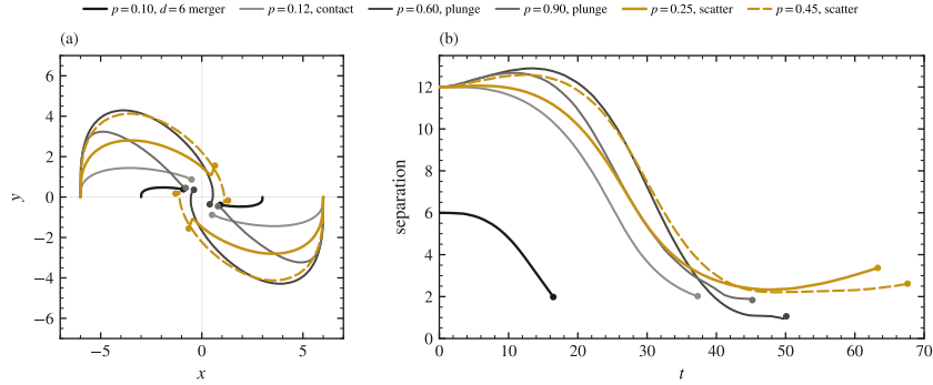
FIG. 12. Merger or fly-by on boosted, solved data: the d = 12 momentum scan and the d = 6 merger. (a) Both throats in the orbital plane; (b) their separation. The tracks are the coordinate positions of the \chi pits, followed through each run by continuity and smoothed over two time units; a track ends (dot) where its pits stop being trackable (a superluminal hop between two \chi minima) or at the run's trust window. Gold: the scatterers, p = 0.25 (solid, to t = 63.3 ) and 0.45 (dashed, to t = 67.6 ). Ink and greys: the plunges p = 0.60 and 0.90 (two legs each, concatenated across their restarts), the d = 6 , p = 0.10 merger, and the p = 0.12 arm, whose pits reach contact at t \approx 37 . Movies: Videos 8 ( p = 0.25 ) youtu.be/fh3pU7xCU_I , 9 ( p = 0.60 ) youtu.be/-ejFKpetL1Y and 10 ( p = 0.90 ) youtu.be/yzvwjC46lJY .
