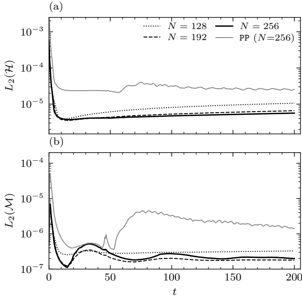
FIG. 10. Constraint norms for the headline cell’s resolution ladder (line styles as in Fig. 6) and the merging PP control at the finest grid (gray). (a) Hamiltonian, L_2 over the domain: finer grids start worse (initial-data interpolation noise) and evolve better. (b) Momentum, L_2 .
