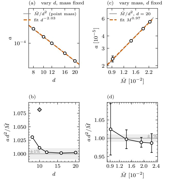
FIG. 5. Both axes of a = \bar{M}/d^2 , measured. Left, mass fixed: (a) fitted acceleration against separation over d_0 = 8\text{--}20 at the base grid (open circles); the power-law fit (orange dashed) gives d^{-2.03 \pm 0.01} , and the point-mass line \bar{M}/d^2 (grey) is indistinguishable from it at this scale. (b) a d^2 over the pair mass \bar{M} : the close-pair excess decays monotonically, gone by d = 16 . The open diamond is the converged ( N = 256 ) value at d = 10 ; the \sim 7\% base-grid calibration is common to the scan and cancels from the exponent and the trend (Sec. VC). Right, separation fixed: (c) the equal-mass ladder at d_0 = 20 —four pairs whose two stars are retuned together, spanning a factor 2.46 in mass—returns a \propto \bar{M}^{0.97 \pm 0.06} against 1 exact. (d) The same ladder compensated: each rung recovers its own mass to within 2.4%, and the residual tilt carries the finite-size sign, the lightest pair being the most diffuse. Error bars are the half-spread of four disjoint-window fits. The ladder is fitted on the halo-free core tracker, which agrees with the whole-domain barycentre to 0.9% on every rung but the lightest, where the shed halo drags the barycentre fit 18% off.
