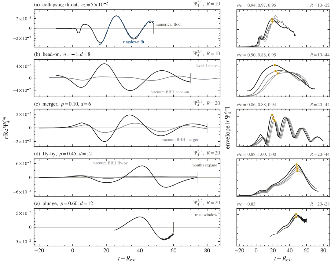
FIG. 7. The waveform gallery: one row per scenario on one retarded clock. Left: r \text{Re} \Psi_4 of the dominant mode at the innermost sphere, each row on its own scale; row (a) is the \varepsilon_2 = 0.05 arm, with the ringdown fit of Sec. VIII A dashed (period 20.6 M ). Caps mark where the drawn record ends: the collapsing throat where its numerical floor passes 10% of the burst peak; the head-on where the noise of its level-1 refinement cube reaches the sphere (from t = 80 at R \leq 20 ); the fly-by at the trough where the mouths' expansion meets the decaying arch ( t - R = 74 ); the plunge at its trust window. The merger runs whole, burst through remnant ringdown. Grey under (b)–(d): the vacuum controls, black holes at the same d and p on bare punctures, on the same scale: the vacuum head-on rings 6.1 \times lower and crests later (Sec. VIII B); the vacuum merger peaks at the drainhole merger's retarded time, 3.0 \times lower; the vacuum fly-by radiates one cycle as the holes swing away from periapsis, 6.7 \times below the fly-by's arch. Right: the amplitude envelope at every sphere on its own retarded time (ink to faint, inner to outer)— |r \Psi_4| for the complex (2, 2) modes, the analytic-signal envelope for the real (2, 0) modes—which folds onto one curve for a signal moving at c and falling as 1/r . Gold dots: the correlated wavefront. The quoted v/c is the whole-waveform lag between neighbouring spheres (Sec. VIII E), the plunge's the burst-peak lag: throat 0.94/0.97/0.95 , head-on 0.94/0.88/0.95 , merger 0.86/0.88/0.94 , fly-by 0.88/1.00/1.00 , plunge 0.83 . Movies of the vacuum head-on and fly-by: Videos 5 youtu.be/aRWvD4W8OOg and 6 youtu.be/65_3kw4obvE .
