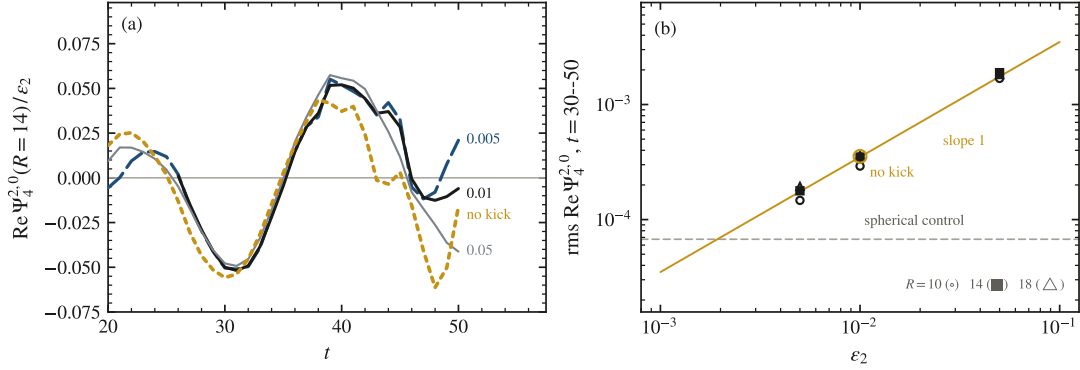
FIG. 11. Linearity of the collapsing throat's wave in its quadrupole seed. (a) \text{Re } \Psi_4^{2,0} at R = 14 , each arm divided by its seed and named at its end: \varepsilon_2 = 0.005, 0.01, 0.05 and the kick-free 0.01 arm collapse onto one curve through the burst; later the smallest arm carries its floor amplified by 1/\varepsilon_2 and the kick-free arm runs ahead. (b) rms amplitude over t = 30\text{--}50 against \varepsilon_2 at three spheres, with the slope-one line through the 0.01 arm drawn across the decade 10^{-3}\text{--}10^{-1} as a reference. Open circle: the pure quadrupole, within 2% of the kicked arm. Dashed rule: the floor of the level-4 spherical control (the same kick, no quadrupole) at R = 14 , which the line crosses at \varepsilon_2 \approx 2 \times 10^{-3} . The outcome: the wave is the quadrupole's—linear in \varepsilon_2 and unchanged, to 2% in amplitude, when the radial kick is removed. The kick alone radiates only the floor; it moves the wave's phase, not its size.
