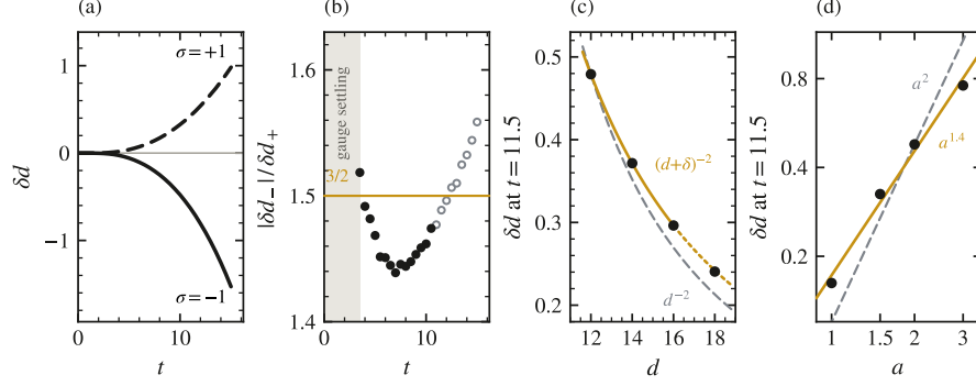
FIG. 4. Two throats at rest, on the far-side-matched pairs (Sec. IID): the sign rule (a,b), the force law (c) and its growth with throat width (d). (a) Separation change of two matched d = 12 pairs one sign apart: like-signed ( \sigma = +1 , dashed) opens, opposite-signed ( \sigma = -1 , solid) closes. Separations are inverse- \chi -weighted centroids of the midplane \chi pits. (b) Pull-to-push ratio against the prediction (Q+1)/(Q-1) = 3/2 (gold), where Q = |F_\phi/F_{\text{grav}}| = (a^2 + m^2)/m^2 = 5 is the scalar-to-gravity force ratio of Eq. (5): measured 1.462 \pm 0.022 (scatter over 15 slices); grey, the gauge-settling window t < 3.5 , excluded; open circles past t = 10.5 , where the closing pair has eaten a tenth of its gap and the displacements are no longer small, excluded too. (c) The force law on the ladder: how far like-signed pairs released from rest at d = 12/14/16/18 have pushed themselves apart by t = 11.5 (dots), against inverse-square in the coordinate separation scaled through d = 12 (grey, dashed) and A/(d + \delta)^2 fitted on d = 12-16 alone (gold), dotted where it predicts the d = 18 rung (Sec. VB). If the push were inverse-square in d , every dot would lie on the grey curve; the dots rise above it, and the gold fit absorbs the excess with the offset \delta . (d) The push against throat width, on logarithmic axes: how far like-signed d = 12 pairs of width a = 1/1.5/2/3 have pushed themselves apart by t = 11.5 (dots; a = 2 is the d = 12 rung of (c)), against the point-charge a^2 of Eq. (5) scaled through a = 2 (grey, dashed) and a power law fitted to all four rungs (gold). If the push grew as a^2 , every dot would lie on the grey line; the dots climb more slowly, as a^{1.4} .
