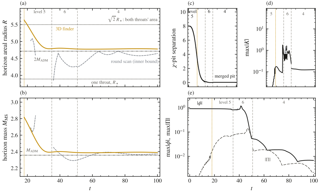
FIG. 5. The head-on merger ( d = 8 from rest, p = 0 , opposite signs) on matched, solved data ( M_{\text{ADM}} = 2.3573 ), and the black hole it makes. One evolution in three legs (faint dashed rules at the seams, t = 35 and 50.8 ; levels named in each panel; Sec. VIB): level 5 to a NaN in h_{11} at the merged core at t = 38.845 , inside the MOTS (its overrun grey to the death cross in (c)–(e)); level 6 from leg 1’s t = 35 checkpoint through the failure window; level 4 to t = 100 with no NaN. In-code \Psi_4 is identical on both overlaps. (a) Areal radius and (b) Misner–Sharp mass of the common MOTS. Gold: the spectral finder’s history (Sec. IIID, one row per plotfile, the three replay legs joined), born at t = 18 with R = 5.634 ( M_{\text{MS}} = 2.817 ) and settling—monotone to 0.08\% per row—onto the Schwarzschild sphere of the pair’s mass: R = 4.7787 and M_{\text{MS}} = 2.3894 at t = 100 , 1.4\% above 2M_{\text{ADM}} and 1.4\% above M_{\text{ADM}} . Grey dashes: the round star scan, the inner bound of Sec. IIID, late and small at birth and blind over t = 26 – 35 (Sec. VIA). Rules: one isolated throat, R_* = 3.8895 ; \sqrt{2}R_* , a sphere with both throats’ area; 2M_{\text{ADM}} ( M_{\text{ADM}} in (b)). (c) Separation of the \chi pits. (d) \max|K| . (e) Grid maxima of |\phi| (solid) and |\text{II}| (dashed): the field is swallowed. Gold dotted rule: horizon birth. Movie: Video 3; youtu.be/3sx9GHRTYVs .
