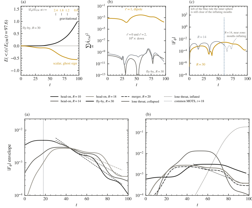
FIG. 13. Top (channel) : The scalar channel on the \Psi_4 spheres. (a) Fly-by energy through R = 30 in units of the gravitational energy crossed by the end of the sphere’s trusted record ( t = 97.6 , t - R = 67.6 ): gravitational (ink) and scalar with its physical sign (gold, Sec. VIII F). The ratio |E_\phi|/E_{\text{GW}} printed at each cut falls from 2.4 at t = 60 to 0.56 over the whole record, as the gravitational burst arrives after the scalar one (Sec. VIII F). (b) Multipole content, fly-by: \ell = 1 exceeds \ell = 0 and \ell = 2 by 10^{6.4} . (c) Validity window: |F_\phi| at both spheres, each drawn to its retarded gate t - R = 67.6 . Past the blue rule ( t = 60 ) the inner sphere reads the inflating mouths’ near field—its climb there has no counterpart at R = 30 one light-crossing later—so that stretch is dashed and carries no claim; the t = 60 window at R = 14 gives 0.6 in place of 2.4. Bottom (censorship) : Envelope of the scalar flux |F_\phi| , horizoned against horizonless arms: a running maximum over 25 units (about one dipole period), smoothed in log amplitude, since the raw flux changes sign every \sim 13 units. (a) The head-on chain’s glued record at R = 10/14/18 . The common MOTS closes at t = 18 (dotted); the remaining hair leaves as one \ell = 1 pulse, cresting later at each sphere, then decays (dashed: fits over t = 30\text{--}95 , \tau = 20/25/32 ). The rise before the rule is the open mouths’ static hair, canonically ingoing; only the post-horizon window is integrated. (b) One sphere per fate (head-on and lone throat R = 18 , merger R = 20 , fly-by R = 30 ): the merger, behind its horizon from t = 13 , decays like the head-on ( \tau = 22 , dotted fit); the fly-by, horizonless, shows its burst’s complete arch, drawn to t - R = 67.6 (its trust window). Mid-grey: the lone throat twice—the \varepsilon = +10^{-2} level-4 collapse (solid), behind a MOTS from t = 11 , and the unkicked level-4 throat (dotted), which inflates, horizonless, and grows in the monopole (counted to t \approx 80 ).
