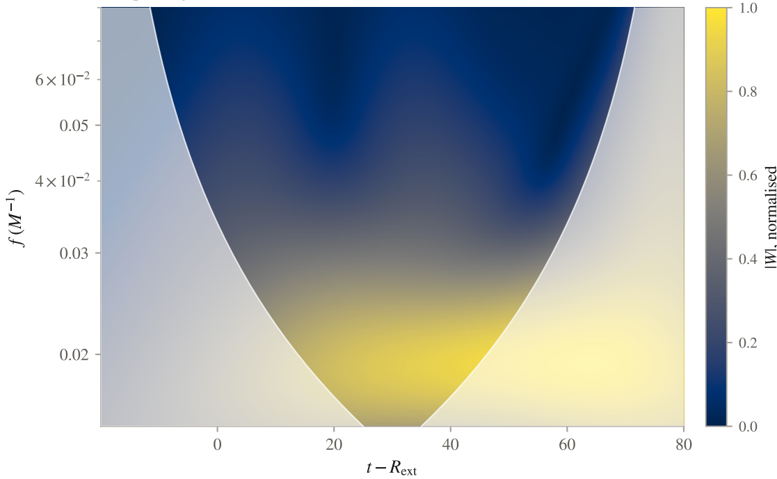
(e) spectrogram at R = 20 (faded: the wavelet overruns the record)
