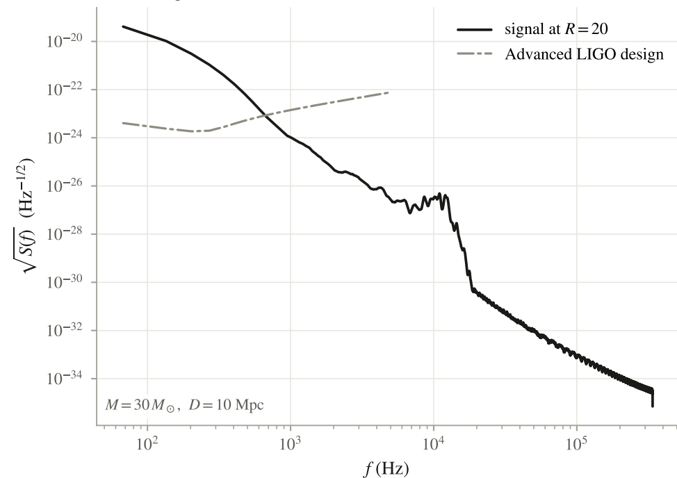
(f) strain against Advanced LIGO
