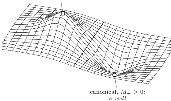
(a) phantom, M_- < 0 : a hill
