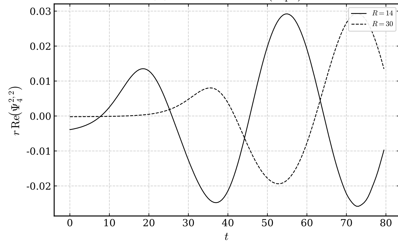
(a) Waveform r \text{Re}(\Psi_4^{2,2})
