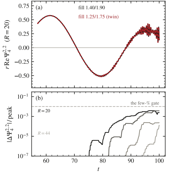
FIG. 10. Moving the fill window does not move the wave. (a) r \text{Re } \Psi_4^{2,2} at R = 20 for the freeze arm (fill 1.40/1.90, ink) and its twin (1.25/1.75, burgundy dots), same t = 57 checkpoint, same binary: one bicolour curve. (b) The per-sphere envelope of the difference against the few-percent gate: at most 0.385% of peak at R = 20 and 0.013% at R = 44 , each front arriving on the fill’s causal clock t = 57 + (R - 1.9) . The figure certifies the fill’s inertness, not a remnant ringdown.
