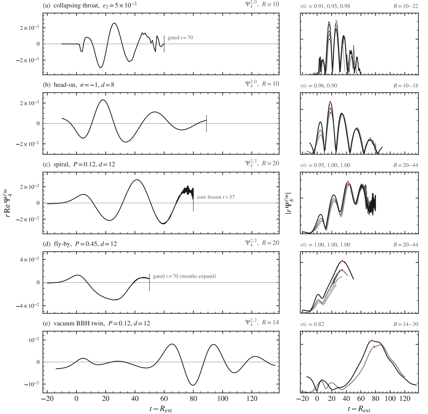
FIG. 7. The waveform gallery: every channel's radiation, one row per scenario, one retarded clock. Left column: r \operatorname{Re} \Psi_4^{\ell m} of the dominant mode at the innermost extraction sphere, each row on its own stated scale—the lone throat radiates an order of magnitude below the mergers, and the fly-by is the loudest channel of all. Half-height caps mark record ends: the collapsing throat's stream is junk-gated at t = 70 , the spiral record ends at t = 60 with the run still in flight, and the fly-by—complete to t = 100 , no horizon ever forming—is gated at t = 70 , ahead of the t = 76.1 trough where the mouths' expansion (areal radii growing \times 7.8 ) has grown to equal the decaying burst at the R = 20 sphere. Right column: the envelope |r \Psi_4^{\ell m}| at every extraction sphere on its own retarded time (ink to faint, inner to outer): a signal travelling at c and falling as 1/r folds onto one curve. Burgundy dots mark the correlated wavefront, and the quoted v/c is the lag of the whole complex waveform between neighbouring spheres over their common retarded window—peak-to-peak timing fails on flat-topped envelopes (the vacuum twin's merger plateau is \sim 15 units wide at both spheres, and its peak times alone would read v = 0.57c where the waveform lag reads 0.82c ). Measured speeds: throat 0.91/0.95/0.98 , head-on 0.96/0.90 , spiral 0.95/1.00/1.00 , fly-by 1.00/1.00/1.00 , vacuum twin 0.82 . Every channel propagates at c within the output cadence: radiation, not a gauge or constraint mode.
