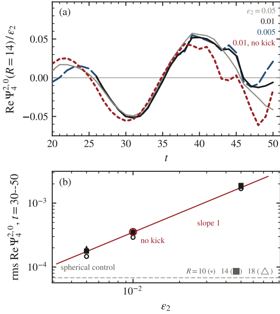
FIG. 9. One throat’s wave is linear in its deformation. (a) \text{Re } \Psi_4^{2,0} at R = 14 , each arm divided by its own seed: \varepsilon_2 = 0.005, 0.01, 0.05 and the kick-free 0.01 arm collapse onto one curve. (b) rms amplitude over t = 30-50 against \varepsilon_2 at three spheres, with the slope-one line through the 0.01 arm: linear to 1–16% across a decade. The open circle is the pure quadrupole—no radial kick—matching the kicked arm to 2–3%; the dashed rule is the spherical control’s floor.
