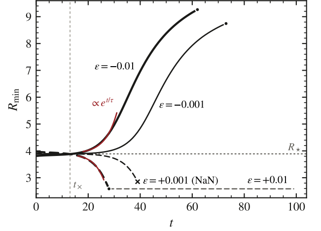
FIG. 2. Declared-seed branching of the lone throat (level 3). Areal throat radius of the drainhole ( a = 2 , m = 1 ; R_* = 3.8895 , dotted) under the kick of Eq. (6): \epsilon = \pm 10^{-2} (heavy), \pm 10^{-3} (light); dashed = outward ( \epsilon > 0 ). The fate is opposite to the push, and each pair crosses itself at the \epsilon -independent t_{\times} \simeq 13.0 —linear response. Burgundy: exponential fits |R - R_*| \propto e^{t/\tau} , \tau = 4.5 ( t = 18 – 31 ) and 4.0 ( t = 16 – 26 )—steeper than the unkicked mode’s 5.88 (Fig. 1) while the kick’s transient decays. Dots: the scan loses the throat (the inflating runs continue to t = 100 , still growing); cross: death at t = 40.1 . The \epsilon = +10^{-2} arm holds a horizon from t = 11 (areal radius 3.88 \rightarrow 2.34 \rightarrow 2.57 ) and runs clean to t = 100 ; the muted line carries its last reading. A tenfold smaller kick arrives 8–12 units later.
