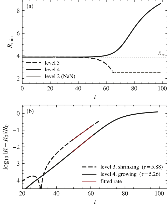
FIG. 1. The undeclared seed: one exact throat, two resolutions. (a) Minimal areal radius of the lone drainhole evolved from exact static data at refinement levels 2–4. The exact solution is a fixed point ( R_* , dotted); each level holds it until its own truncation error excites the unstable mode, and the fate flips with the grid: level 3 (dashed) collapses, level 4 (solid) inflates. Level 2 (grey) dies of an origin failure at t = 24.2 (cross) with the throat still exact to 0.12%—too coarse to reach the branch at all. Dot and muted line as in Fig. 2: the scan loses the level-3 throat at t = 65 while the run continues to t = 100 behind a marginally trapped surface (areal radius 3.23 \rightarrow 2.37 ). (b) The deviation grows exponentially on both grids: plateau fits over t = 49 – 61 give e-fold times \tau = 5.88 (level 3) and 5.26 (level 4)—the same unstable mode to 9%, T = \tau \alpha_{\text{th}}/R_* = 0.87 and 0.78 against the González-Guzmán-Sarbach band 0.68 – 0.76 [14]—with opposite sign. The fate is the truncation seed’s; the mode is the throat’s.
