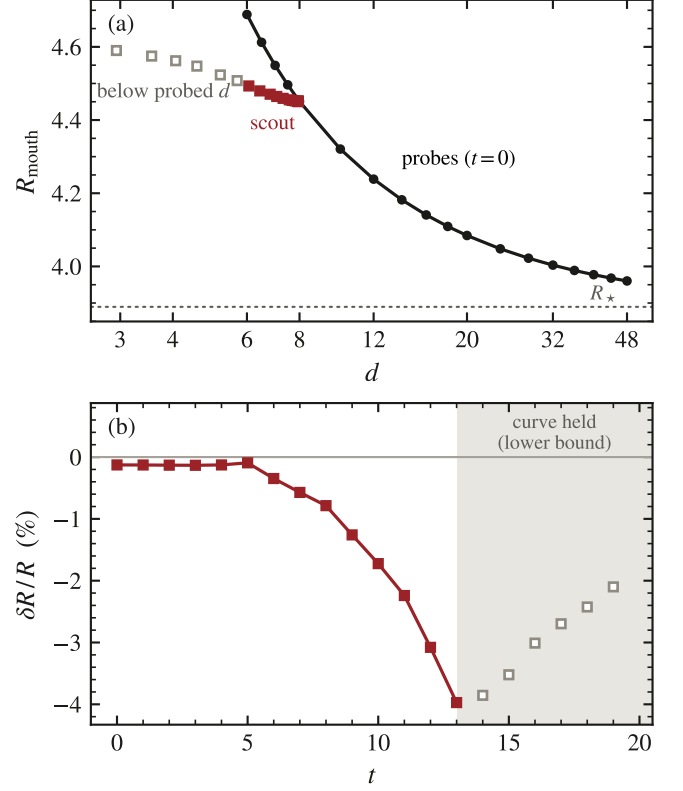
FIG. 4. Placement is on the ruler; the squeeze is not. (a) Per-mouth areal radius of two exact drainhole throats placed at rest, read at t = 0 by one-step probes at separations d = 6\text{--}48 (ink): the pair reads wider than the isolated throat ( R_* , dotted), the excess falling as d^{-1.16} —the neighbour’s field on the ruler, not a dynamical widening. Burgundy squares: the head-on scout’s mouths (the \sigma = -1 pair released from rest at d = 8 , Sec. VI) at the separation it had reached; open squares, here and in (b): the scout closer than the closest probe. (b) The scout against the curve at its own separation, \delta R/R = R_{\text{scout}}/R_{\text{place}} - 1 . The -0.13\% plateau to t = 5 is the mouth tracker’s grid snap ( d reads 7.94 for a true 8) and calibrates the systematic; the throats’ own squeeze then grows to -4.0\% by t = 13 ( d = 6.1 ). In the band the curve is held at its last point, so the magnitude is a lower bound—the apparent recovery is the ruler’s, not the throats’. A boost can only raise a coordinate-sphere reading, so a reading below the curve is a real squeeze, if anything underestimated.
