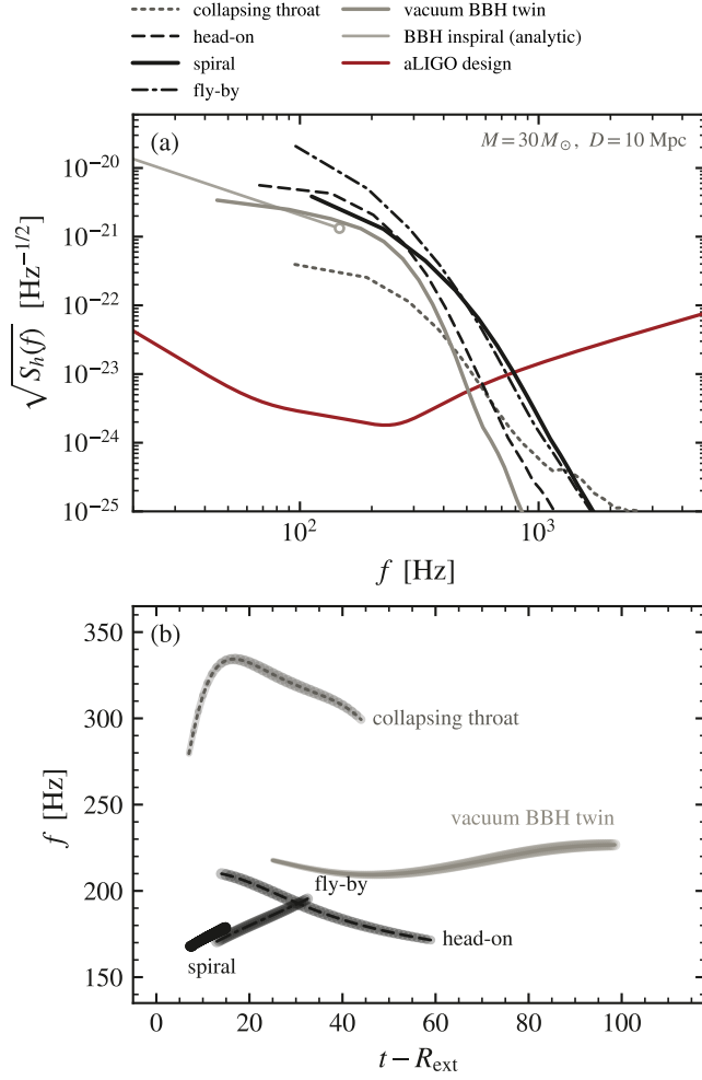
FIG. 6. Every source on a detector, at one shared calibration: total mass M = 30 M_\odot , distance D = 10 \text{ Mpc} ; strain scales as M/D and frequency as 1/M . (a) Strain amplitude spectral densities of the innermost-sphere records over the aLIGO design floor (burgundy). Every channel clears the floor around 100 Hz: the fly-by peaks at 2.1 \times 10^{-20} \text{ Hz}^{-1/2} (96 Hz); the head-on, spiral and vacuum twin lie within a factor of two of one another ( 3.4\text{--}5.6 \times 10^{-21} ); the lone collapsing throat sits an order below ( 3.9 \times 10^{-22} ). The faint straight line is the analytic Newtonian inspiral of the same equal-mass binary, |\tilde{h}(f)| \propto \mathcal{M}^{5/6} f^{-7/6} , drawn to its ISCO at 147 Hz through the same normalisation as the numerical record: the ramp an astrophysical binary rides into the band where the simulated signal begins. (b) Peak-frequency tracks of the Morlet wavelet transform of each record (the line's width is the signal's own envelope; tracks are drawn only above 0.2 of each record's peak and outside the cone of influence). The shapes separate the sources: the collapsing throat rings in an arch at 280–334 Hz, the head-on bell slows from 210 to 170 Hz, the vacuum twin climbs through merger onto a 227 Hz ringdown shelf, and the spiral and fly-by (records in flight) enter as rising arcs at 165–195 Hz.
