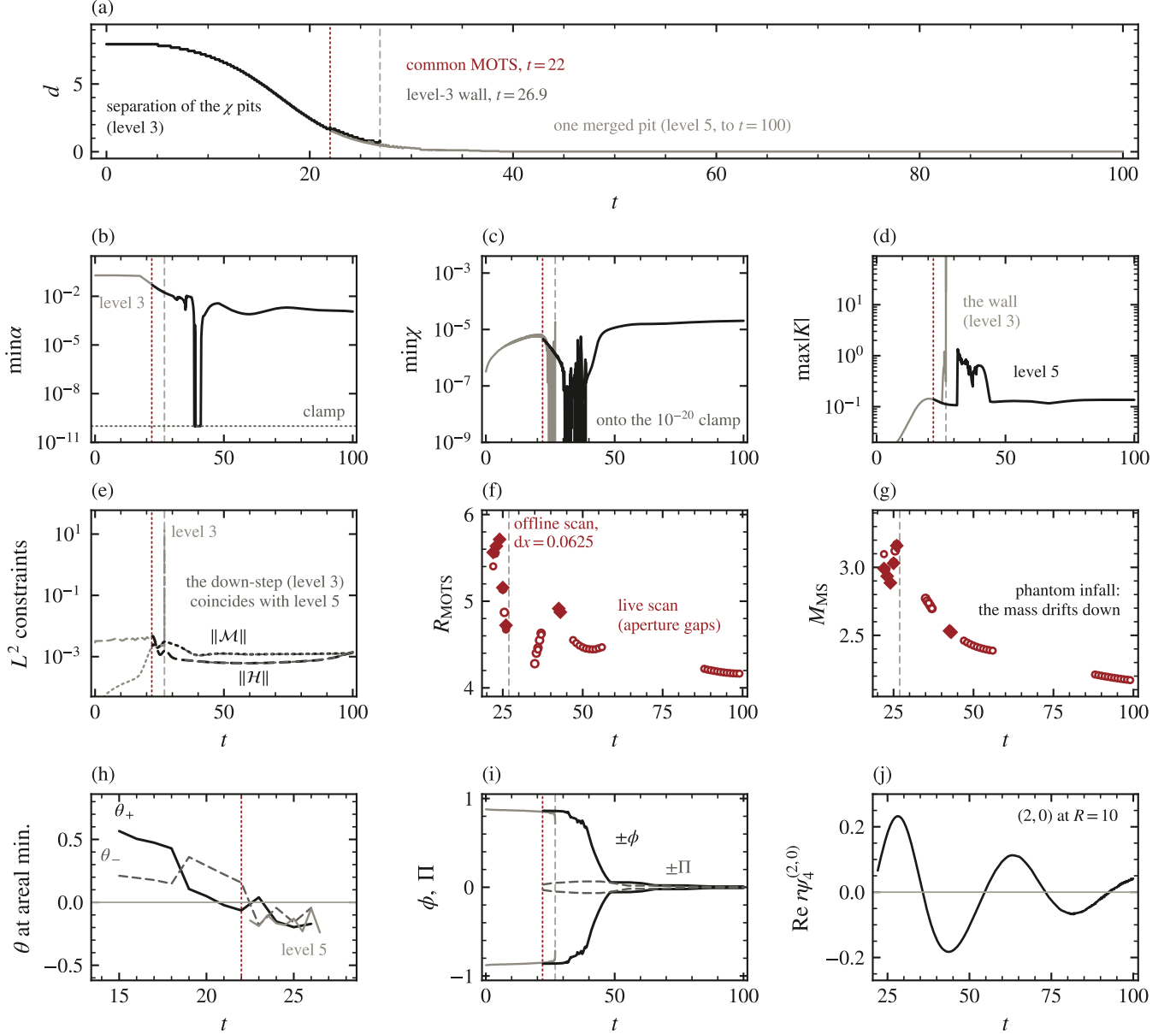
FIG. 4. The head-on merger makes a black hole ( d = 8 from rest, opposite scalar signs); every horizon point is the orientation-corrected scan. (a) Separation of the \chi pits: level 3 carries the formation from d = 7.94 (the tracker's grid snap on a true 8); the common MOTS forms at t = 22 (burgundy rule in every time panel), the scout dies at the level-3 wall at t = 26.91 (dashed rule), and the level-5 arm, restarted at t = 22 with every interior device off, carries the merged pit to t = 100 with no NaN. (b) The minimum lapse (level 5, ink) rides the 10^{-10} clamp over t = 38.5\text{--}41.0 and settles at 1.1 \times 10^{-3} . (c) Minimum \chi : excursions onto the 10^{-20} clamp leave the frame; level 5 returns and settles at 2.0 \times 10^{-5} . (d) The wall is resolution: \max|K| blows up to 18 at the level-3 death; level 5 never exceeds 1.34 and ends at 0.14. (e) The scout's \|\mathcal{H}\| explodes at the wall (13.6); the level-5 norms fall 4.6 \times 10^{-3} \rightarrow 1.4 \times 10^{-3} ; the down-step (level 3 again, from the t = 35 checkpoint) lands on them to median 0.08%/1.5%. (f) The horizon: filled diamonds, offline scans at dx = 0.0625 (formation at t = 22 , r = 3.17 , R = 5.56 ; growth to 5.71 by t = 24 ; then 4.72, and 4.92/4.87 at t = 42.5/43 ); open circles, the live scan on three arms. Its gaps are aperture, not horizon loss—the shells reach 0.5d + 2.3 , so once the pits merge the surface at r \simeq 2.7\text{--}3.3 lies outside while every shell within reports trapped; where two arms see it at once they agree ( t = 36 : R = 4.461 against 4.441). (g) The Misner–Sharp mass drifts down, 2.99 at formation to 2.17 at t = 99 ( -0.0066 per unit): phantom infall removes mass. (h) Expansions at the areal minimum: \theta_+ crosses zero between t = 20 and 21, both negative by t = 24 ; the per-mouth scans never find an own MOTS—the horizon is born common. (i) The field's extrema fall \pm 0.86 \rightarrow \pm 0.008 with |\Pi| \leq 0.07 : the supporting scalar is swallowed and radiated, leaving vacuum around a black hole. (j) The remnant's (2, 0) mode at R = 10 rings with period \sim 31\text{--}38 , \times 0.6\text{--}0.8 per half-swing, as the mass in (g) declines.
